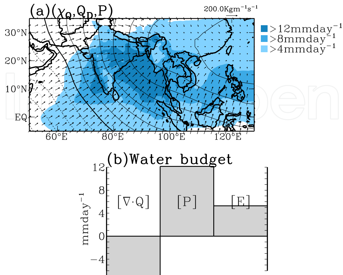
Fig. 2. (a) Summer-mean potential function of water vapor flux ( \chi_Q ), the divergent water vapor flux ( \bar{Q}_D ), and precipitation ( P ). Contour interval is 2 \times 10^9 \text{ m}^2 \text{ s}^{-1} \text{ g kg}^{-1} for (a). The analysis domain used in (b) was marked as a thick black box in Fig.1(b).
