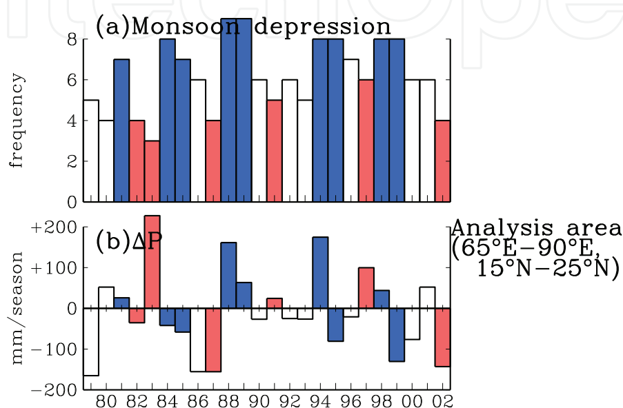
Fig. 12. Histogram of occurrence frequency of the MD at each year from 1979 to 2002 in (a), and total monsoon rainfall over the northern India (65°E – 90°E and 15°N – 25°N) in (b). Warm and cold years of the eastern Tropical Pacific was indicated by red and blue colors. This was based on SST anomaly over the NINO3 region (150°W – 90°W and 5°S – 5°N).
