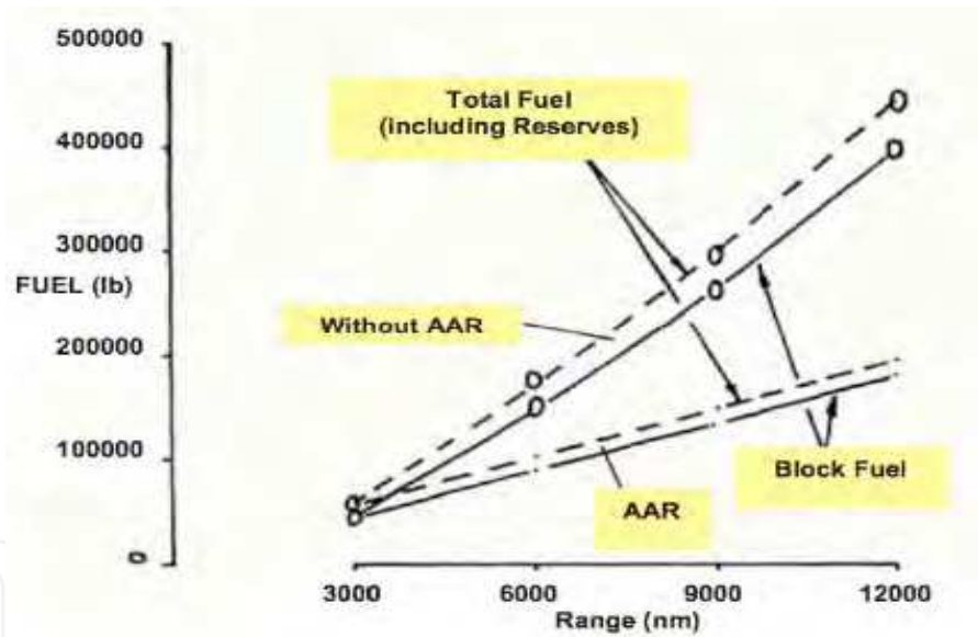
Fig. 28. Savings in fuel burn with Air-to-Air Refuelling (AAR) for long haul flights [31].
