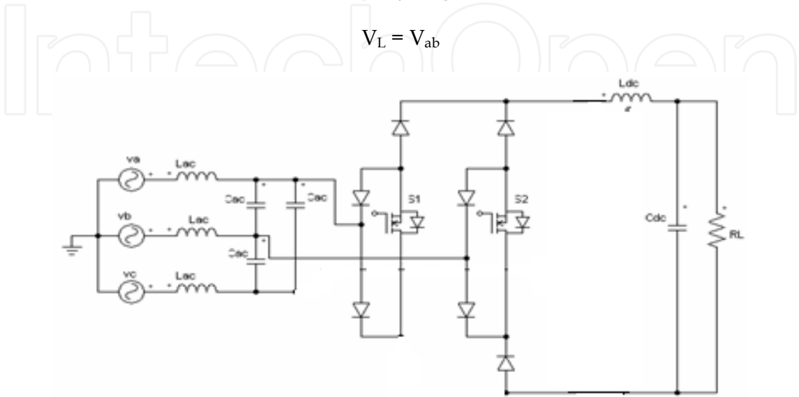
Fig. 6. Mode 1 equivalent circuit.
