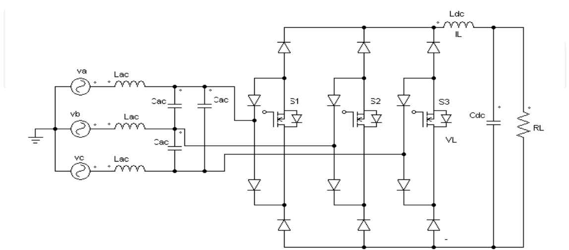
Fig. 4. Buck converter.
