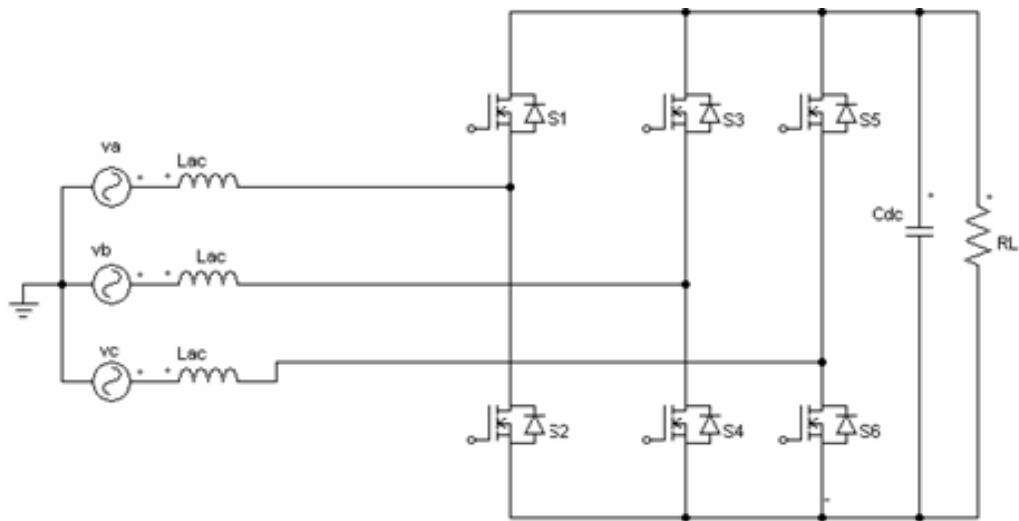
Fig. 1. Boost converter.
