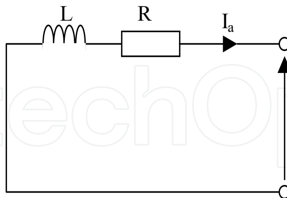
Fig. 13. Schematic of current control for the boost converter.
