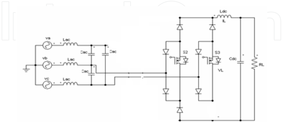
Fig. 7. Mode 2 equivalent circuit.
