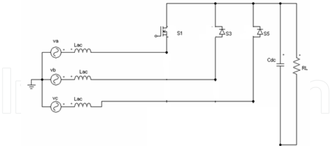
Fig. 3. Boost converter when V_a is negative.
