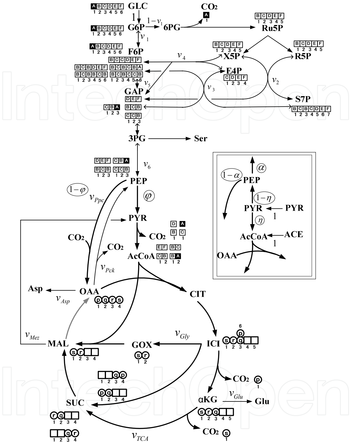
Fig. 8. Main metabolic pathways in the central metabolism together with the fate of [1-^{13}\text{C}] glucose.
