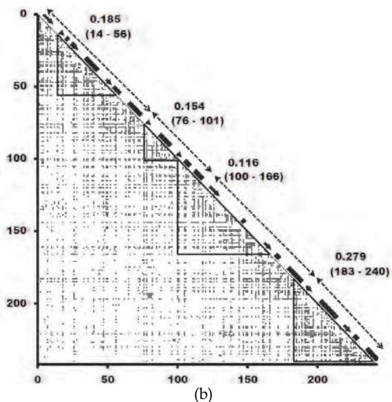
Fig. 4. ADMs for (a) HisF and (b) HisA. A bar along the diagonal denotes a position of a \beta -strand and an arrow does that of an \alpha -helix. A region of a predicted folding unit is enclosed by solid lines in a map with a parenthesis and a numeral denotes the \eta value corresponding to the corresponding predicted region. A broken double arrow means the portion of a corresponding (\beta\alpha)_2 unit.
