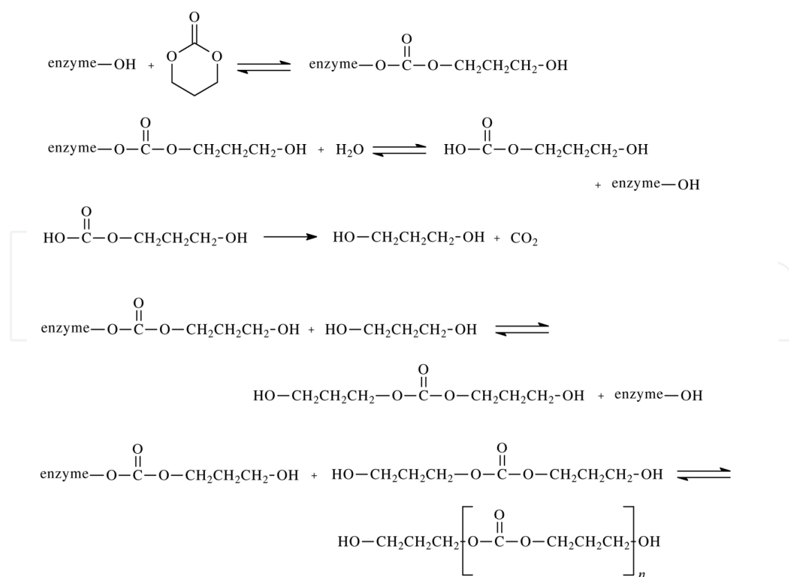
Scheme 2. The mechanism of e-ROP of cyclic carbonates
