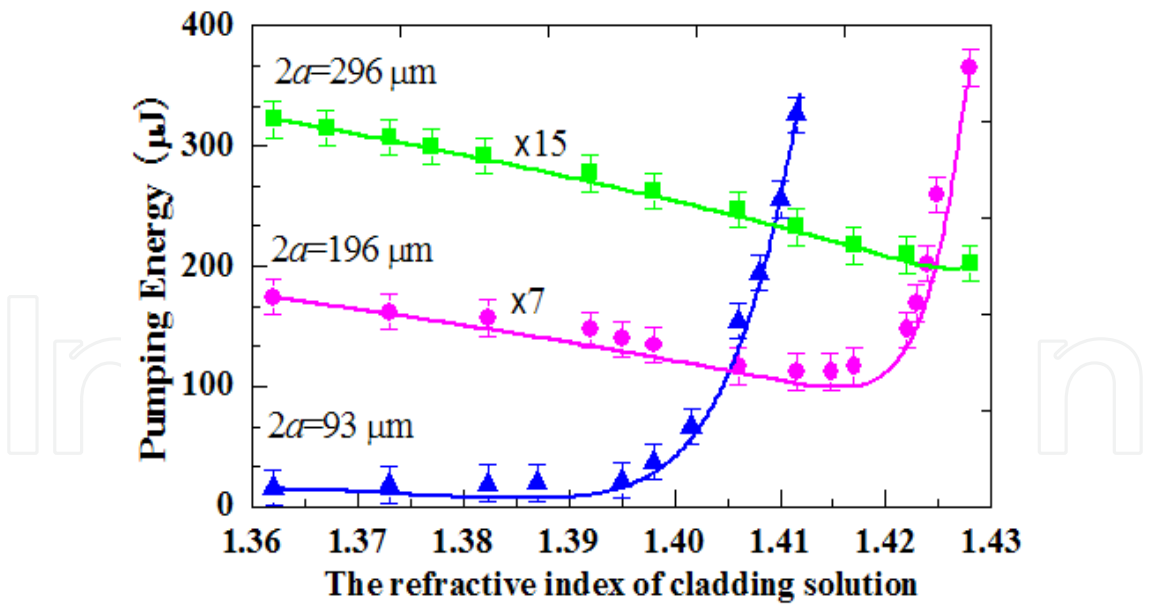
Fig. I-6. Threshold energies varied with the refractive index of cladding solution at the position of Z = 0\text{ mm} . Green square points: experimental data for the fiber of diameter 296 \mu\text{m} , red circle points: experimental data for the fiber of diameter 196 \mu\text{m} , blue triangle points: experimental data for the fiber of diameter 93 \mu\text{m} . Solid curves: theoretically calculated results.
