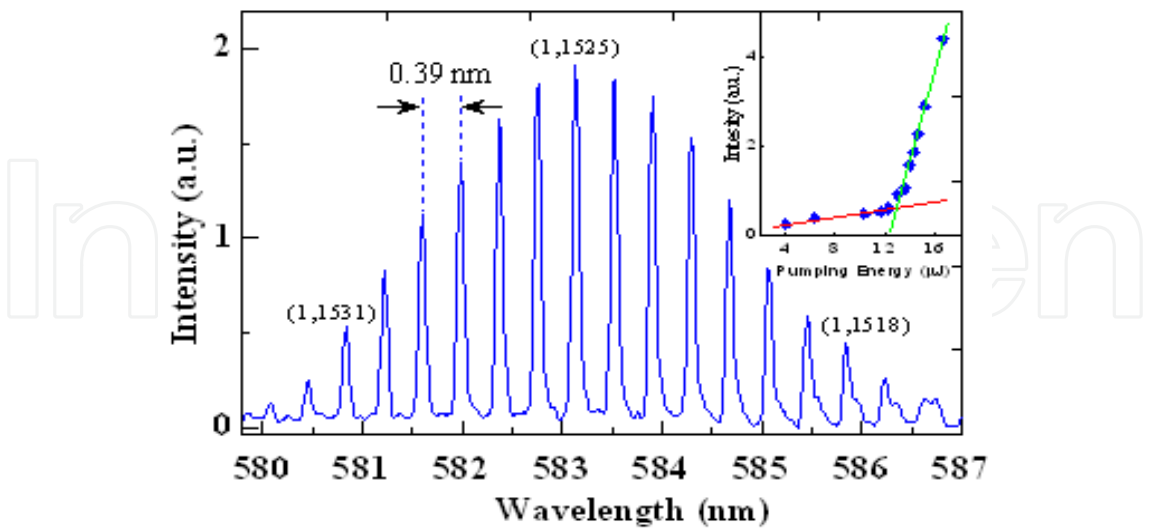
Fig. I-5. Lasing spectrum from the WGM fiber laser of a fiber diameter 196 \mu\text{m} . The output intensities of the laser versus pump energies are shown in the insert of the figure. The measured free spectral range is 0.39 nm indicated by a pair of arrows, and the assigned modes for each lasing peaks are indicated by brackets.
