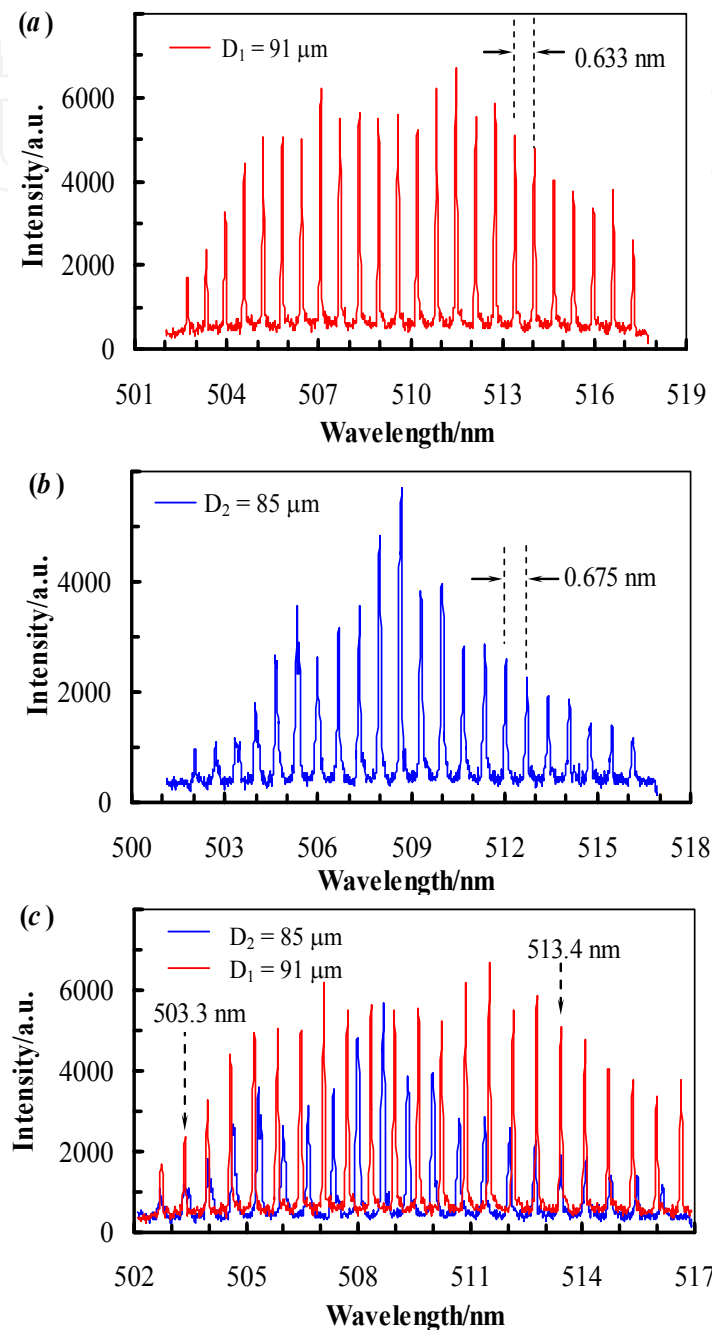
Fig. IV-2. WGM fiber lasing spectrum from a bare optical fibre of diameter D_1 = 91 \mu\text{m} is shown in (a), the measured FSR is 0.633 nm as indicated by the arrows. The spectrum from the bare optical fibre of diameter D_2 = 85 \mu\text{m} is shown in (b), the measured FSR is 0.675 nm as indicated by the arrows. The combination of spectra (a) and (b) in the same wavelength region is shown in (c). Two arrows in (c) indicate the overlapping positions of the WGM resonant wavelengths of the two fibers.
