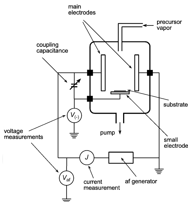
Fig. 3. A schematic diagram of the three-electrode AF reactor.
