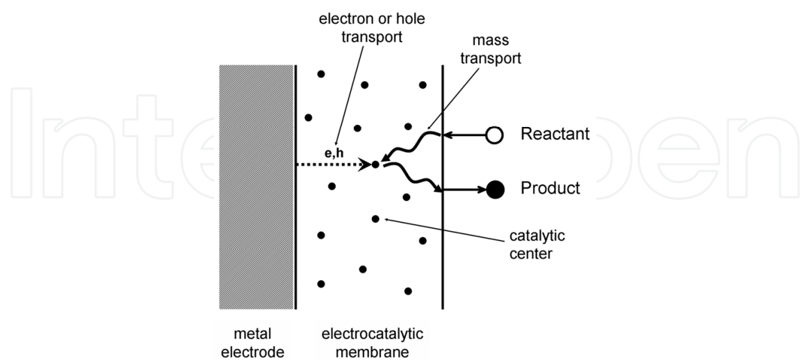
Fig. 10. Model of a three-dimensional (3D) electrocatalytic membrane (Tyczkowski, 2010).
