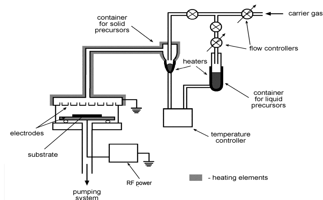
Fig. 2. A sketch of a typical parallel plate plasma reactor.
