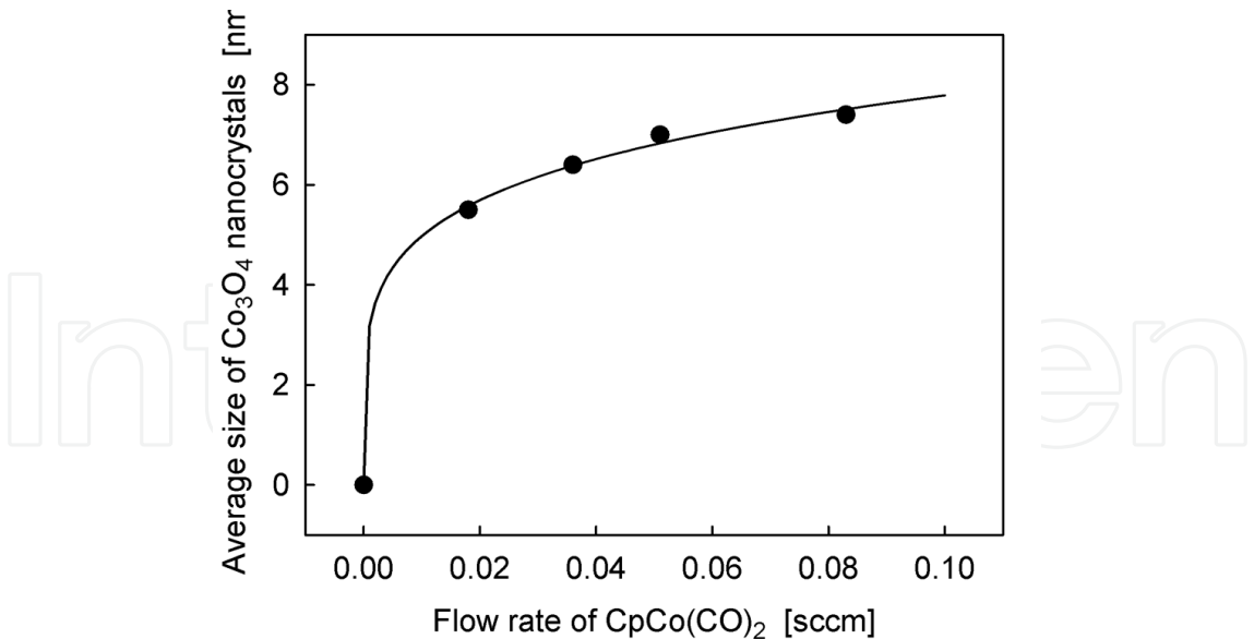
Fig. 12. Dependence of the average size of \text{Co}_3\text{O}_4 nanocrystals on the flow rate of \text{CpCo}(\text{CO})_2 vapor through the plasma reactor (Tyczkowski, 2011).
