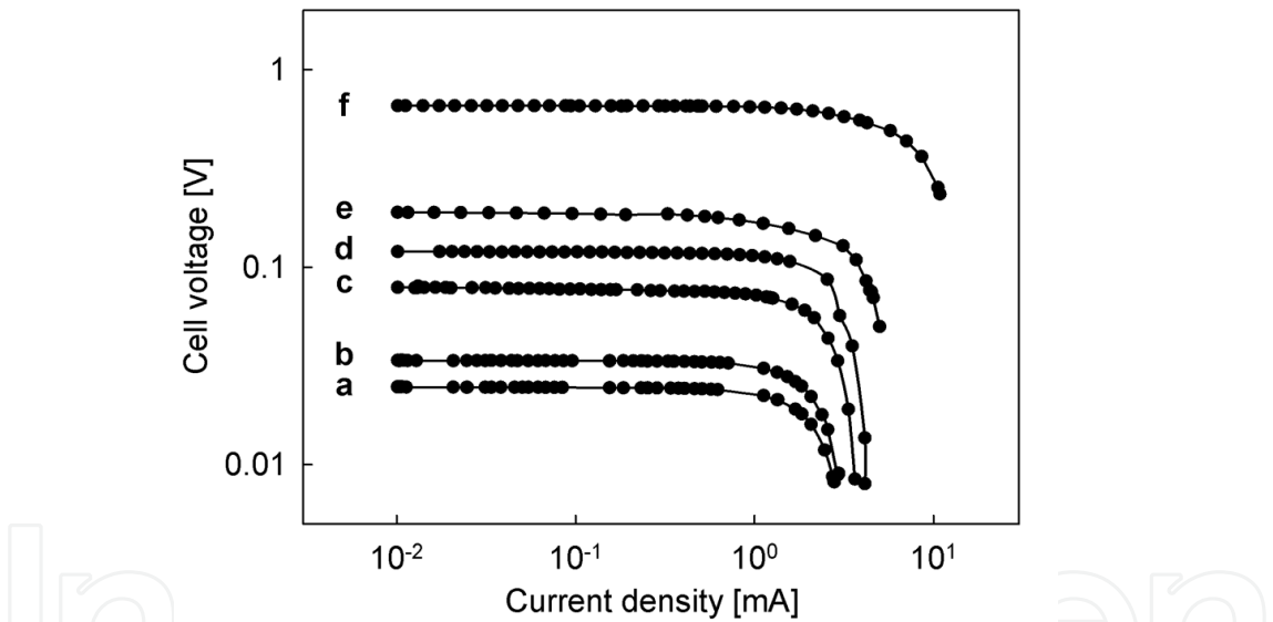
Fig. 13. Fuel cell characteristic for various cathode catalytic materials: (a) – \text{CuO}_x ( t = 12 min); (b) – \text{Co}_3\text{O}_4 ( t = 12 min); (c) – \text{Co}_3\text{O}_4 + \text{CuO}_x ( t = 12 min); (d) – \text{Co}_3\text{O}_4 ( t = 60 min); (e) – \text{Co}_3\text{O}_4 ( t = 80 min); (f) – Pt (Tyczkowski, 2011).
