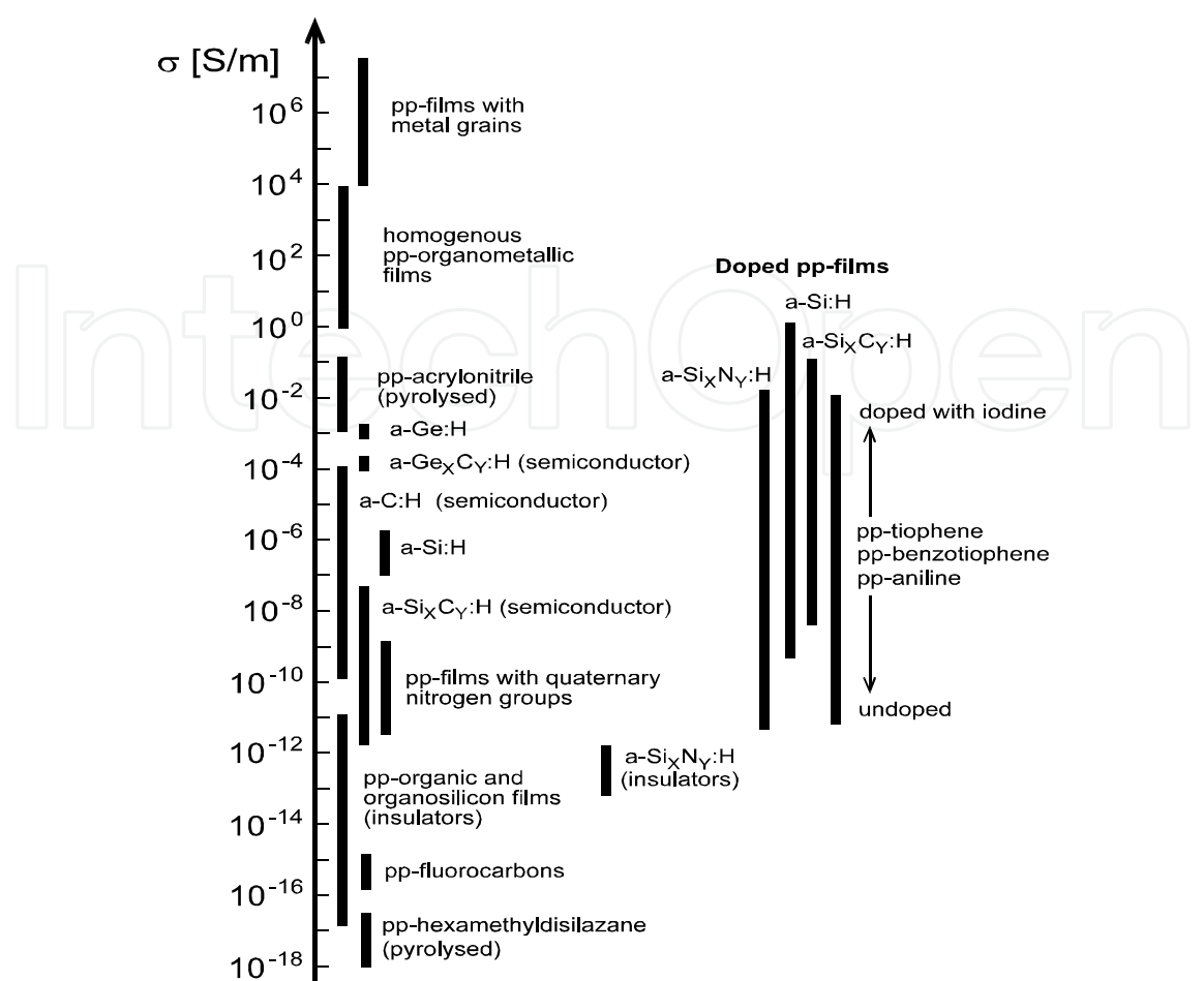
Fig. 9. Room-temperature conductivity \sigma of the main groups of plasma polymers (Tyczkowski, 2004).
