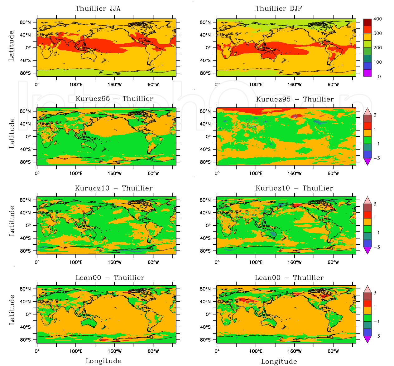
Fig. 8. Compared in the upper panels are the surface temperature distributions determined by the ACCESS model for two seasons using the reference solar spectrum with those determined using the model spectra displayed as separate differences in the bottom panels.
