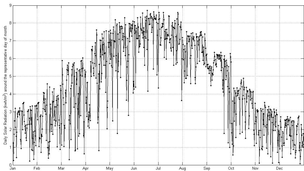
Fig. 3. Daily solar radiation (kwh/m 2 ) around the representative day of each month for the 20 year period (1985-2004), in the city of Athens, Greece.
