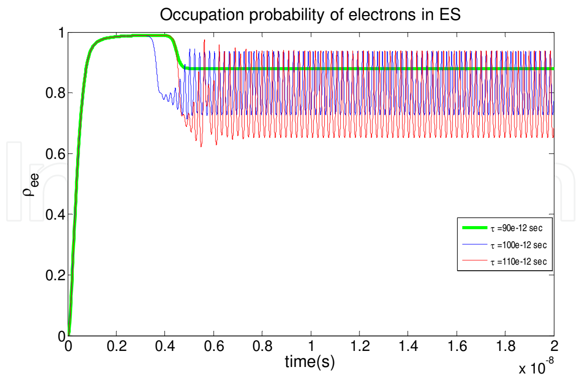
Fig. 4. Time series of electron occupation probability in ES at three values of time delay when J_{cl}=1.5 J_{th} , \phi =0 , \alpha=2 and \gamma=0.025e12 .
