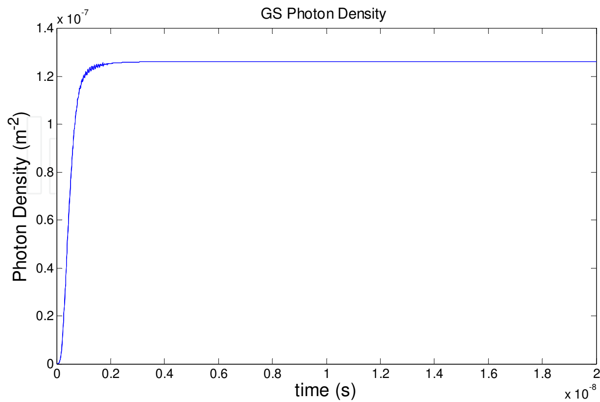
Fig. 2. Time variation of Photon density in GS when J_{c1}=1.5 J_{th} , \text{fi}=0 , \alpha=2 and \gamma=0.025 \times 10^{12} .
