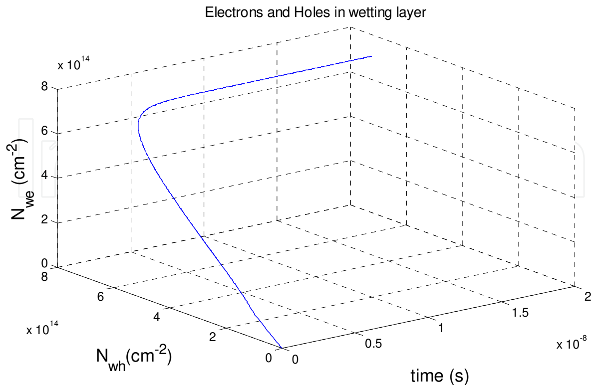
Fig. 5. 3D plot of WL electron and hole densities at J_{cl}=1.5 J_{th} , \phi=0 , \alpha=2 and \gamma=0.025e12
