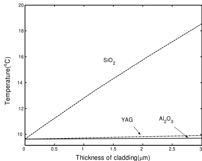
Fig. 2.4. The highest temperature in the waveguide verses coating thickness for Al 2 O 3 , YAG and SiO 2 coatings when pump power is 1 kW.
