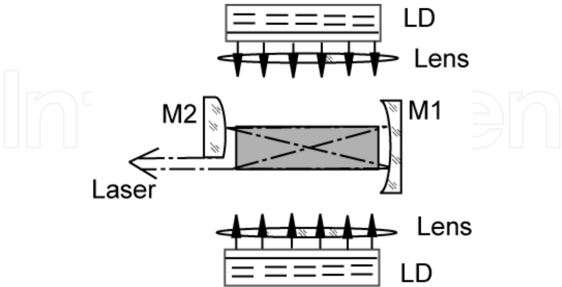
Fig. 2.6. Installation of non-symmetrical Nd:YAG planar waveguide laser.
