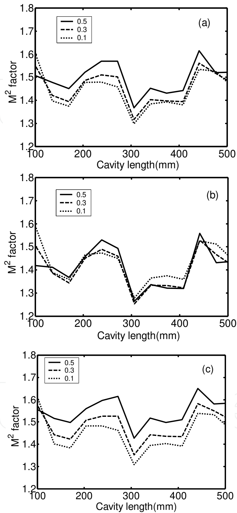
Fig. 1.6. Beam propagation factor M^2 values with symmetric pumping (a) and with asymmetric pumping of b = 1.5 (b) and b = 0.6 (c).
