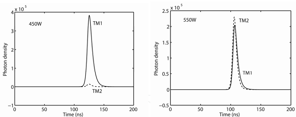
Fig. 2.17. Temporal profiles of TM1 and TM2 modes with pump power of 450 W and 550 W, respectively.
