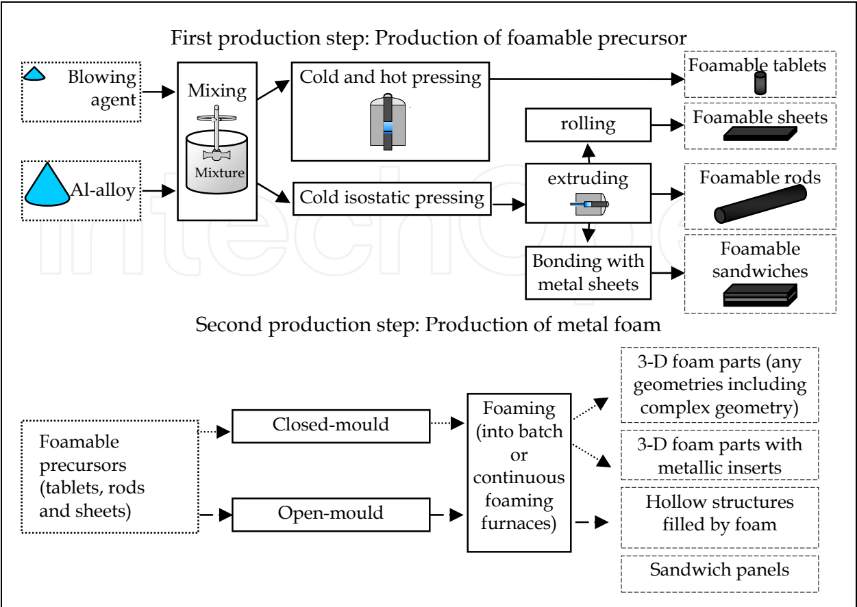
Fig. 1. Powder Metallurgical metod for making metal foams.
