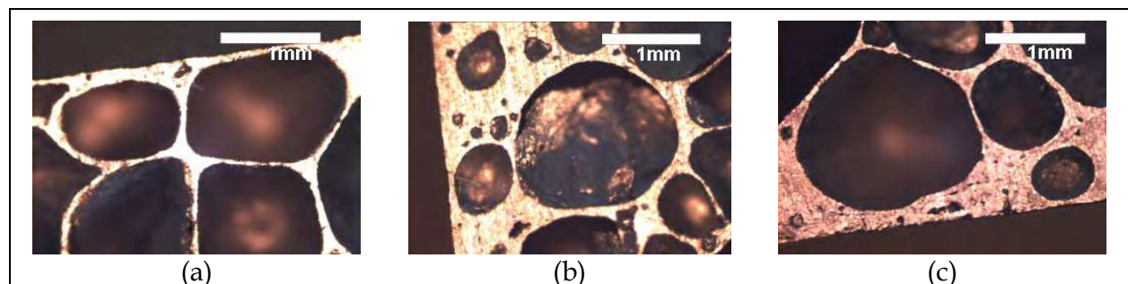
Fig. 22. Thicknesses of the dense surface skin in different sections a sample AlSi7 foam: (a) top, (b) lateral and (b) bottom sides.
