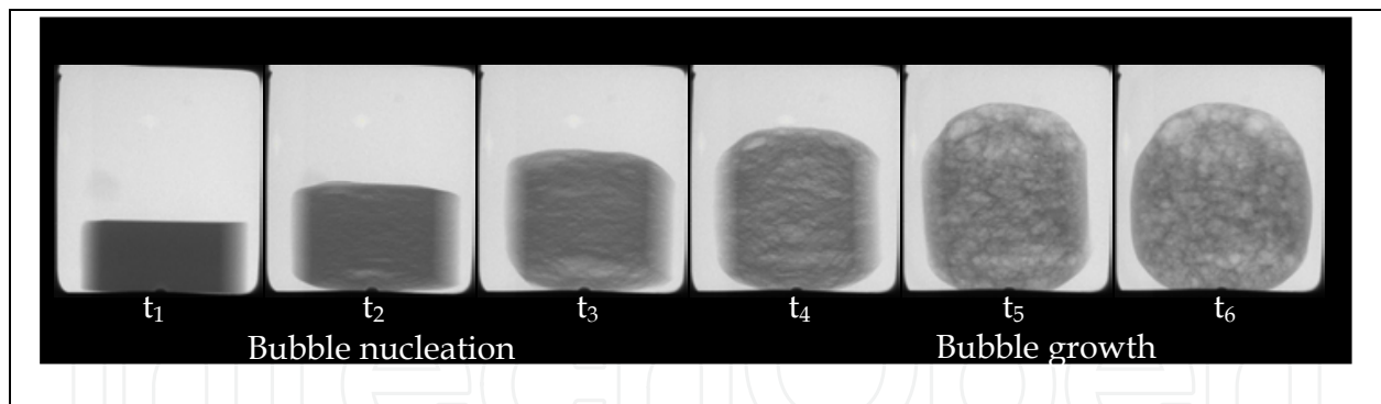
Fig. 19. In-situ radioscopic images acquired during a foaming process of a precursor.
