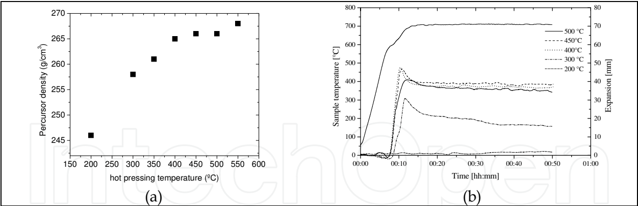
Fig. 10. Effect of the hot pressing temperature on the precursor density (a) and on the foaming behaviour (b).
