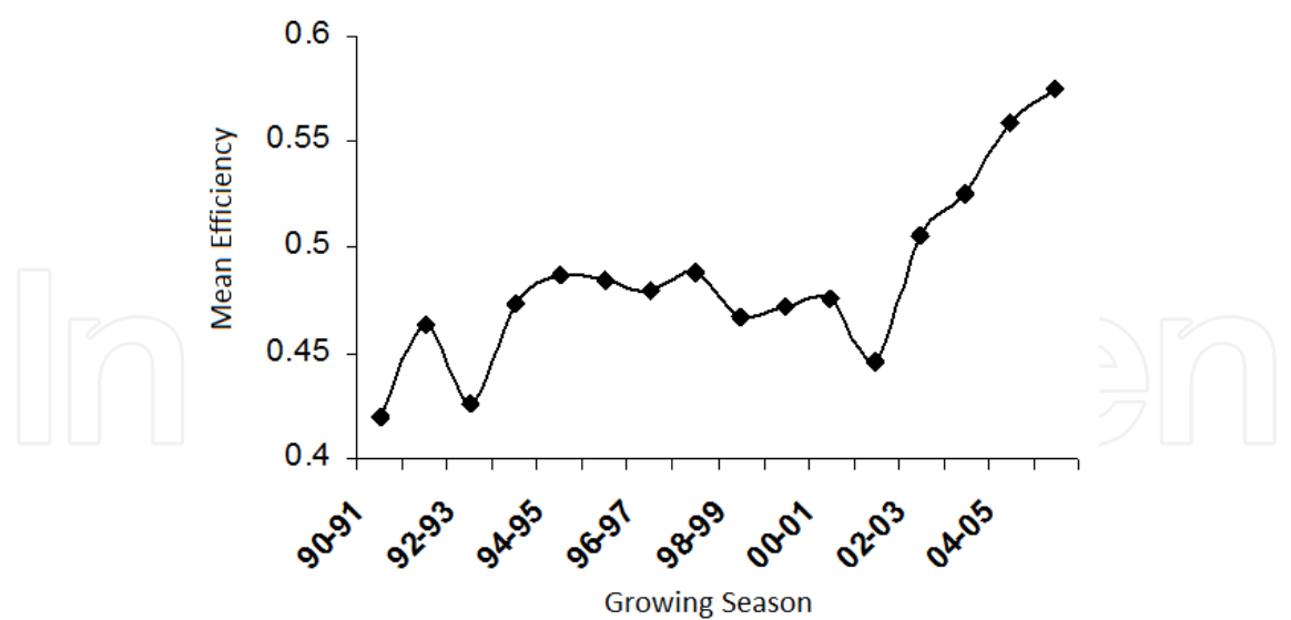
Fig. 2. Time variation of sugarcane production efficiency in the State of Sao Paulo between seasons 1990/1991 and 2005/2006.
