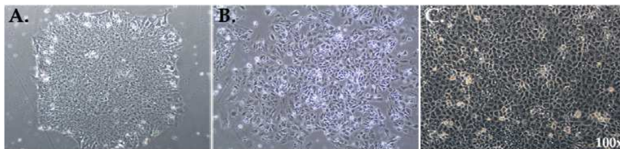
Fig. 3. Examples of iPSC in vitro . A. undifferentiated iPSC colony; B. a spontaneously differentiating iPSC colony; C. iPSC cell-derived hepatocytes formed after following an in vitro protocol adapted from Si-Tayeb et al. 2010. All cells were cultured on matrigel in mTeSR1 media
