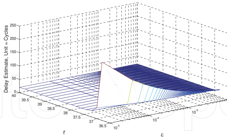
(a) Delay Estimates with \varepsilon and r
