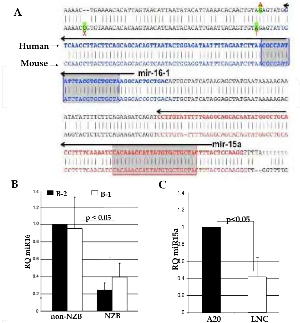
Fig. 2. Identification of Point Mutation and Deletion in miR15a/16-1 Flanking Region: A) Wild type sequence of human (top row) and mouse (bottom row) miR15a/16-1 and its flanking region is shown. The mature miR15a sequence is in red and mature miR16-1 sequence is in blue. Sequencing of this region led to the discovery of an A to T point mutation and deletion of C (40bp upstream of miR16-1) in NZB mice. A homologous A to G point mutation was found in a subset of CLL patients. The substituted nucleotide is written below the corresponding wild type base and the deletion is indicated by an 'X'. B) Spleen cells from NZB and non-NZB mice were sorted into B-2 (IgM+B220+) and B-1 (IgM+B220dull). The expression of mature miR16 in the sorted cells was measured using TaqMan miR-16 Assay according to manufacture's instructions. Data from three independent sorts was analyzed using student's t test ( p < 0.05 ). C) The expression of mature miR15a was compared between the NZB derived cell line LNC and a non-NZB derived B cell line A20 using TaqMan miR-15a Assay. Data from three independent experiments was analyzed using student's t test ( p < 0.05 ).
