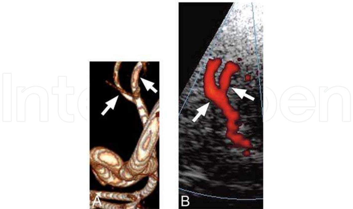
Fig. 7. MRA (a) and TCCS (b) showing a bipode division with a good correlation between the two techniques
