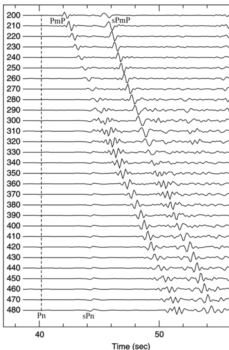
Fig. 5. Synthetic waveforms generated with depth 12 km, azimuth 236^\circ , at distances 2.0^\circ to 4.8^\circ . Top trace 200 was generated at distance 2.0^\circ . Traces are aligned on Pn . The sPn phase stands out at 3.0^\circ (trace 300), but is buried at closer distances. After 2.8^\circ (trace 280) waveforms become complex. Around trace 410 ( 4.1^\circ ) waveforms are simple again.
