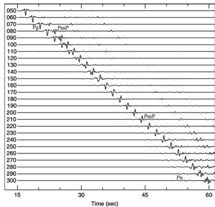
Fig. 11. Synthetic waveforms generated with depth 13 km, an explosive source model, and crustal model 1 in Table 1, at distances of 0.5° to 3.0°. Trace 210 was generated at 2.10°. The Pg phase disappears at about 1.5° (trace 150). The PmP phase is clear from 1.7° to 2.8° (traces 170 to 280).
