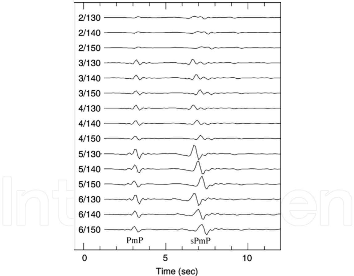
Fig. 10. Synthetic waveforms generated with the five crustal models listed in Table 1 at distance 2.10° and with depths 13, 14, and 15 km. Trace Group 2 (2/130, 2/140, 2/150) was generated with a two-layer crustal model (Model 5 in Table 1); Group 3 with a three-layer crustal model (Model 4 in Table 1); Group 4 with a four-layer crustal model (Model 3 in Table 1); Group 5 with a five-layer crustal model (Model 2 in Table 1); Group 6 with a six-layer crustal model (Model 1 in Table 1).
