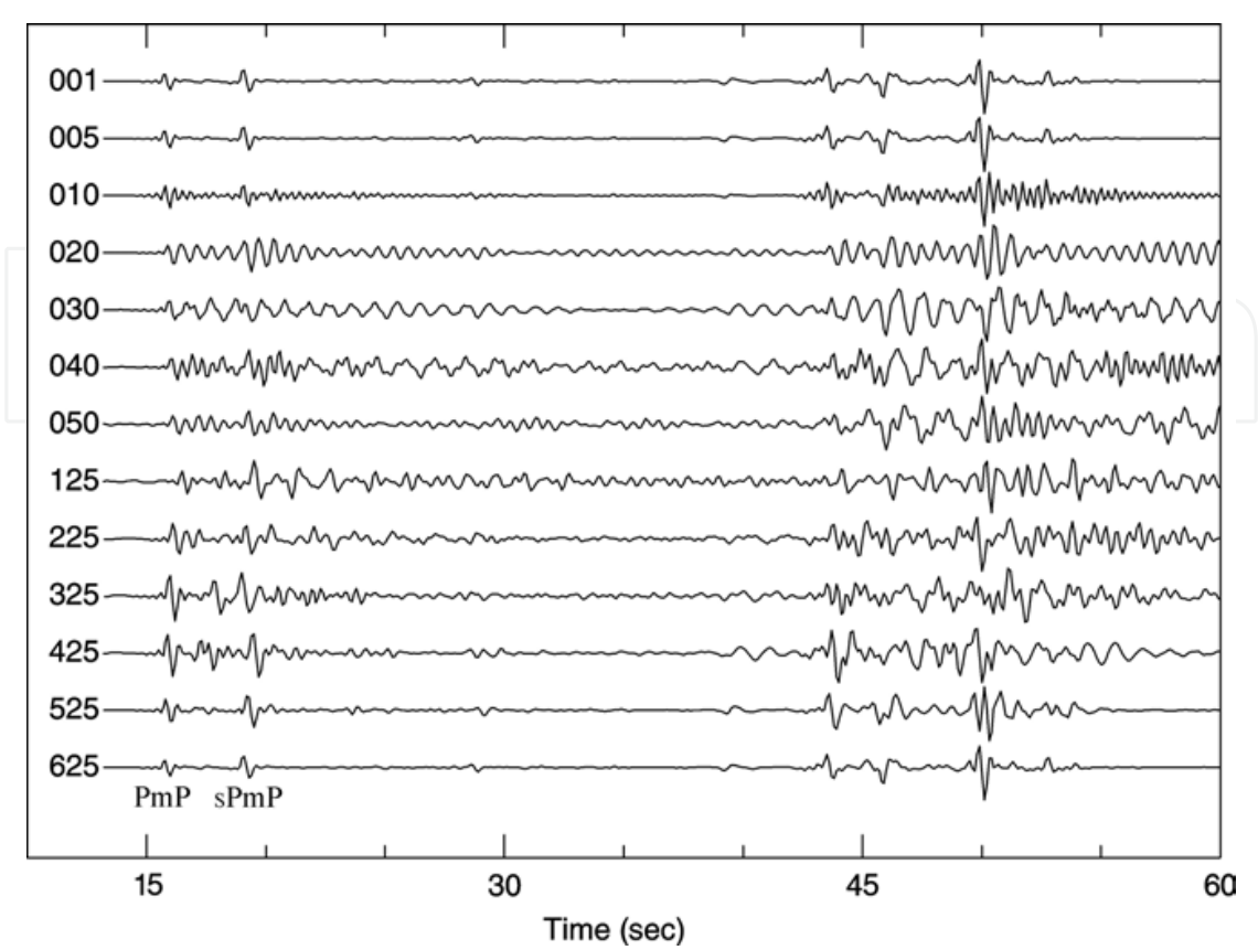
Fig. 20. Synthetic waveforms generated with the new crustal models listed in Table 2 at distance 2.20° and depth 12 km. Trace 125 was generated with Model 1 in Table 2; trace 225 with Model 2; trace 325 Model 3; trace 425 Model 4; trace 525 Model 5; trace 625 Model 6. Trace 001, 005, 010, 020, 030, 040 and 050 were generated with Model 1, but the thickness of the first layer was changed in steps to 0.01, 0.05, 0.1, 0.2, 0.3 0.4, and 0.5 km, successively.
