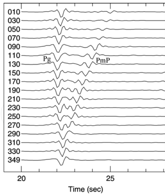
Fig. 12. Synthetic waveforms generated at distance 0.8° with depths of 1.0 to 34.9 km, an explosive source model, and crustal model 1 in Table 1. Trace 130 in this figure is the same as trace 080 in Fig. 11. Because the total path length becomes shorter with focal depth, the PmP phase arrives progressively earlier with depth.
