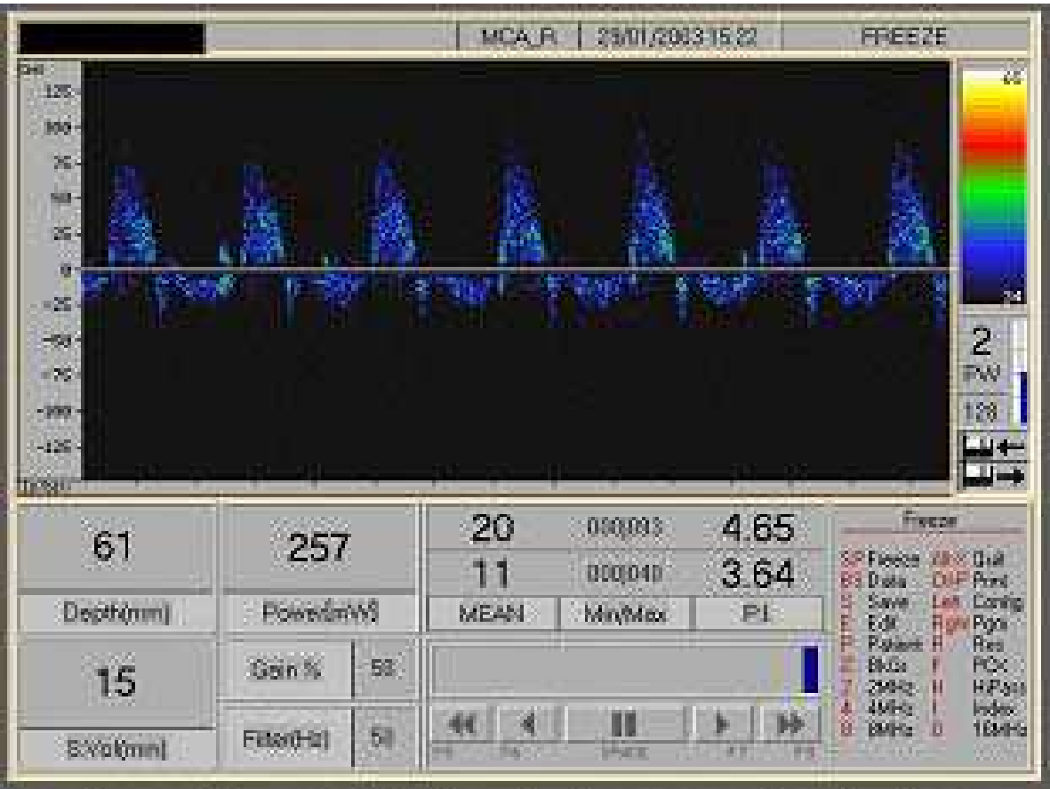
Fig. 6. Oscillating flow in middle cerebral artery (MCA)
