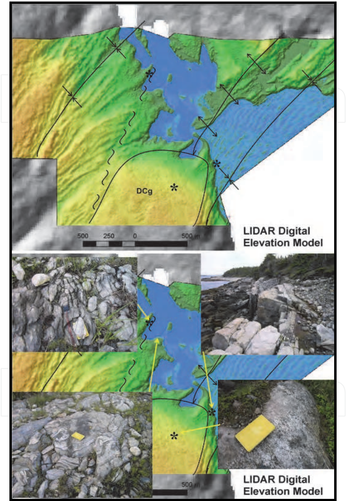
Fig. 15. Top: new interpretation of fold structures and contact between the Goldenville Formation (sedimentary rocks) and granite (DCg large dome to south). Bottom: field photos of rock outcrops that support the interpretation.
