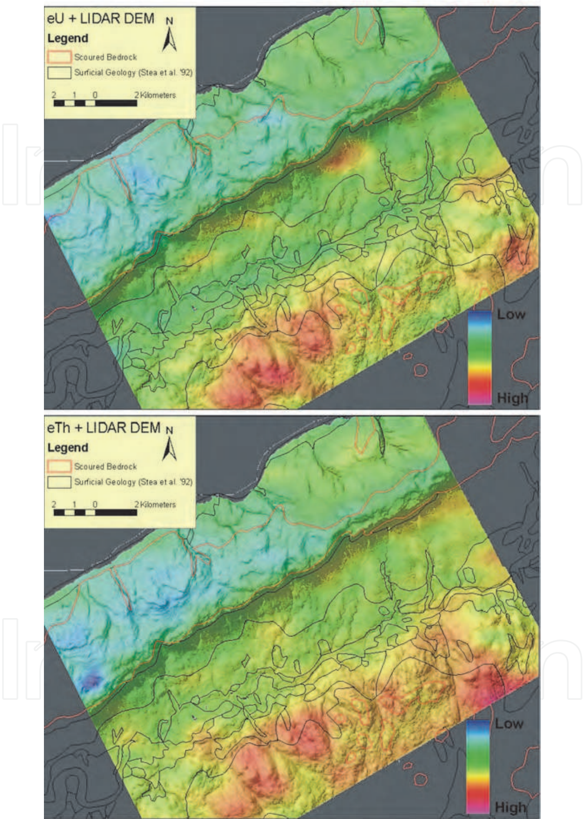
Fig. 8. Radiometric equivalent uranium (top) and thorium (bottom) have been colourized and merged with the lidar shaded relief maps. Low concentrations are colour coded blue through higher concentrations in red. The red areas on the south side of the valley correspond with granite bedrock.
