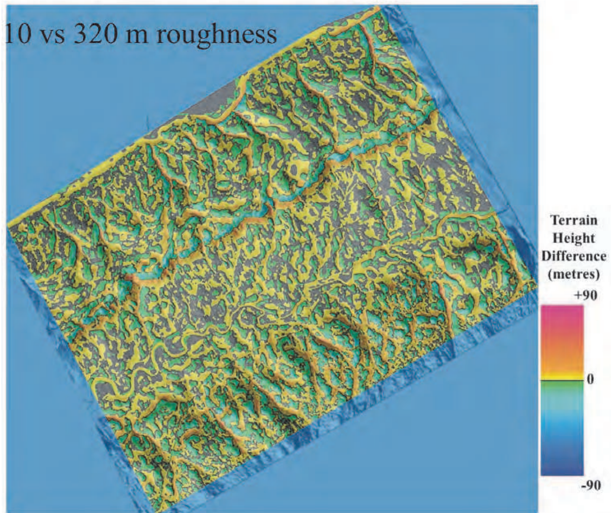
Fig. 25. Example of roughness grid difference between topographic scale 320 m and 10 m. Note the drumlins and streamline glacial landforms are highlighted in the valley floor as well as some of the basalt flow unit boundaries on the North Mountain.
