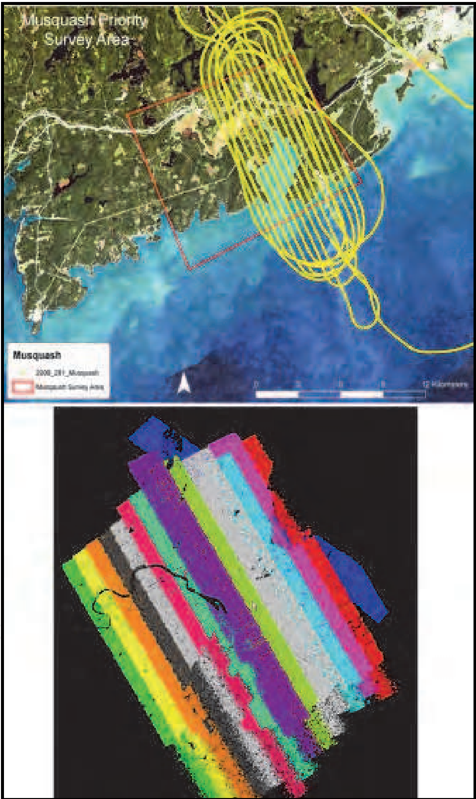
Fig. 2. Top map shows the flight trajectory of the aircraft during a lidar survey, yellow dots. The bottom map shows the lidar swaths associated with the above flight lines. Note the black outline of the river where no returns were detected because of the smooth mirror like surface of the water. Musquash, New Brunswick, Canada.
