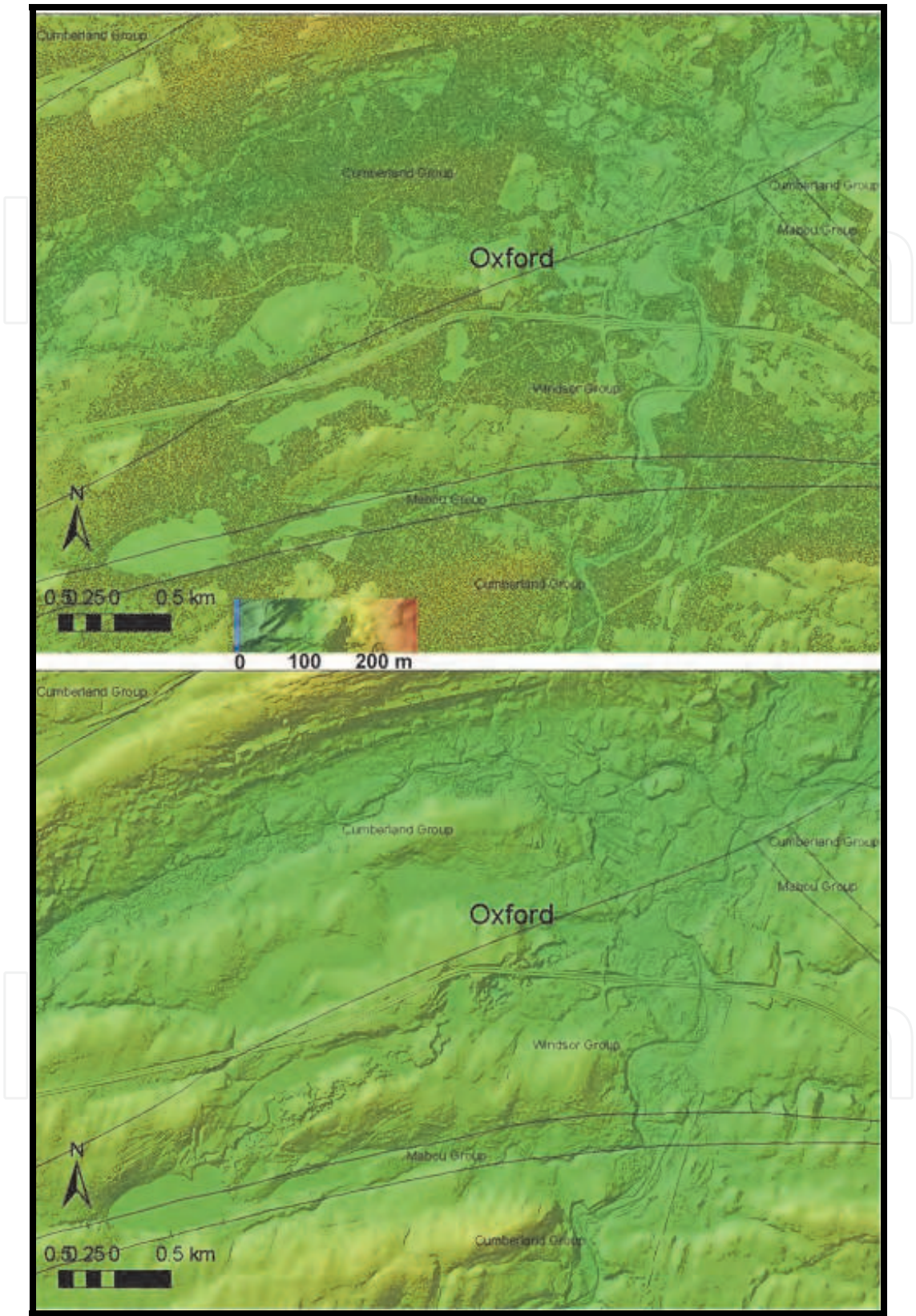
Fig. 16. Top Lidar DSM CSR of Oxford with geological boundaries. Bottom: Lidar DEM CSR with sink holes and karst topography developed below the town of Oxford. Geological boundaries (Keppie, 2000).
