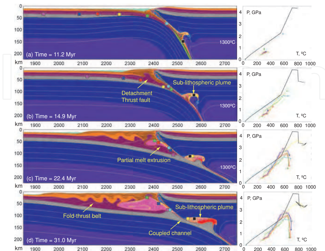
Fig. 6. Enlarged domain evolution ( 900 \times 225 \text{ km} ) of the model with higher temperature of the oceanic lithosphere (hot model). Colors of rock types are as in Figure 1. Time (Myr) of shortening is given in the figures. White numbered lines are isotherms in ^{\circ}\text{C} . Small colored squares indicate positions of representative markers (rock units) for which P - T paths are shown (right). Colors of these squares are used for discrimination of marker points plotted in P - T diagrams and do not correspond to the colors of rock types.
