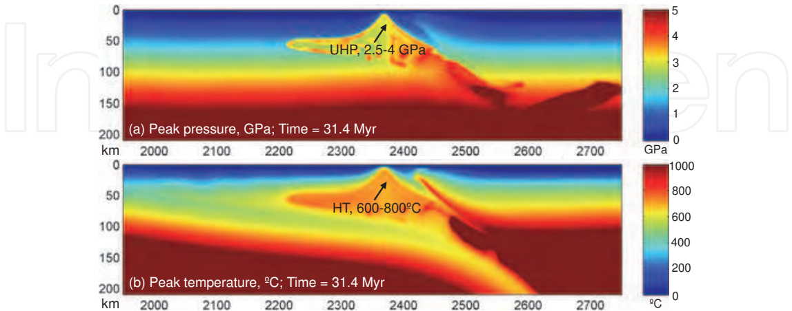
Fig. 3. Peak metamorphic conditions of the reference model. (a) Peak pressure condition in \text{GPa} ; (b) Peak temperature condition in ^{\circ}\text{C} .
