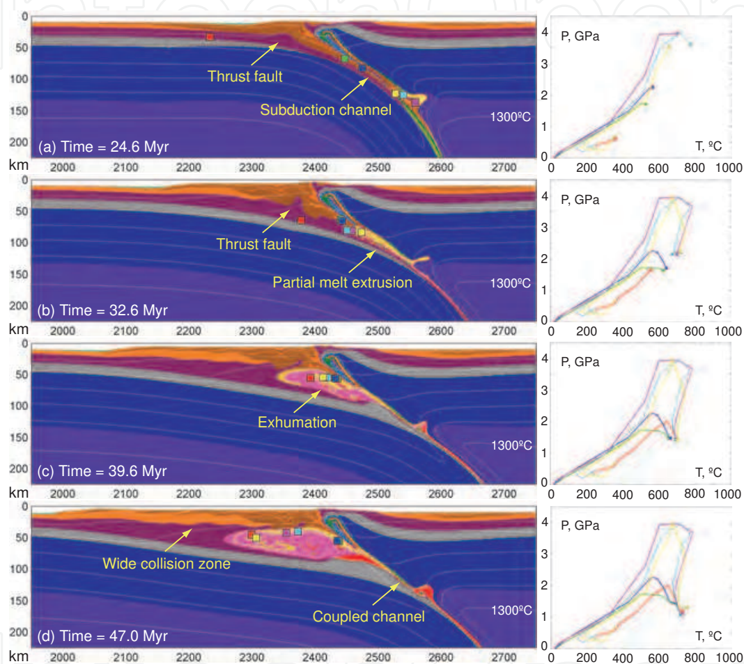
Fig. 4. Enlarged domain evolution ( 800 \times 225 \text{ km} ) of the model with lower convergence velocity V_x = 2.5 \text{ cm/y} . Colors of rock types are as in Figure 1. Time (Myr) of shortening is given in the figures. White numbered lines are isotherms in °C. Small colored squares indicate positions of representative markers (rock units) for which P - T paths are shown (right). Colors of these squares are used for discrimination of marker points plotted in P - T diagrams and do not correspond to the colors of rock types.
