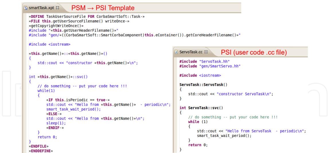
Fig. 17. PSM to PSI transformation of the SMARTTASK. Left: Excerpt of the transformation template ( xPand ) generating the PSI of a standard task. Right: The generated code where the user adds the business logic of the task.
