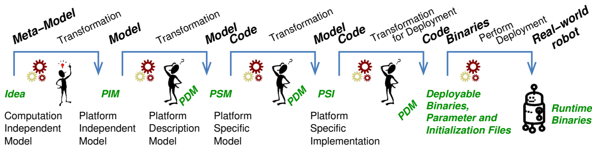
Fig. 5. Model-driven software development at a glance.
