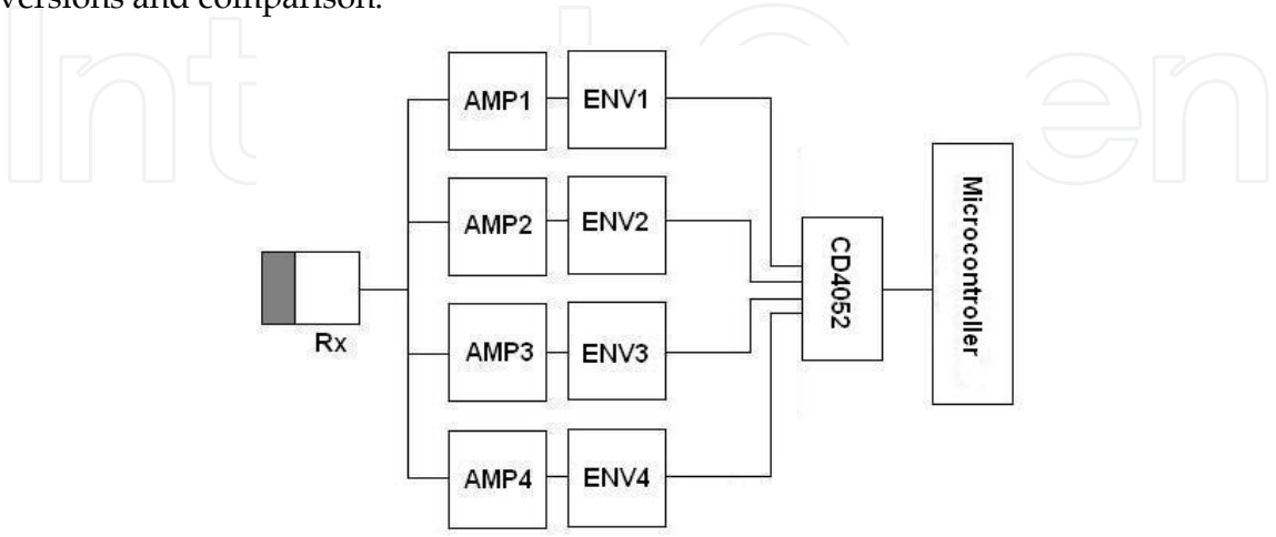
Fig. 4. Electronic circuit for calculating an estimated value of A. AMP1, AMP2, AMP3 and AMP4 are the same as in Figure 3. ENV means envelope detector
