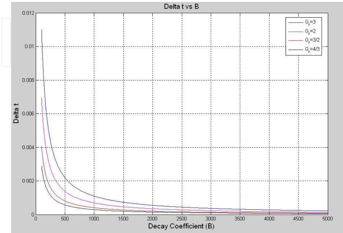
Fig. 2. Behavior of the duration increment of the time interval, ( \Delta t ), in function of the decay coefficient for values of G_1=10, 20, 30 and G_2= 20, 30, 40
