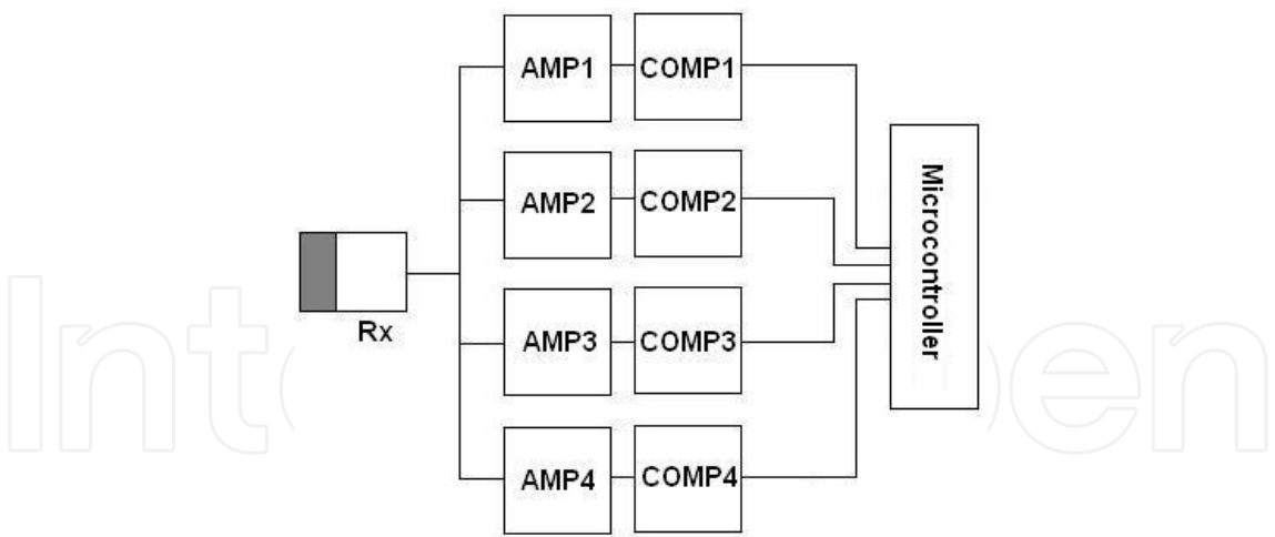
Fig. 3. Clustering circuit to assure that the A value is similar in signals which are compared in terms of duration of the time interval. The abbreviation Amp refers to the amplifier and Comp to the comparator
