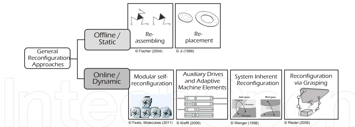
Fig. 2. General classification of reconfiguration approaches to adapted parallel robots to external environments.
