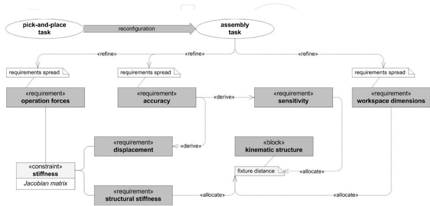
Fig. 15. Relation network for the static reconfiguration of a tow DoF parallel mechanism.
