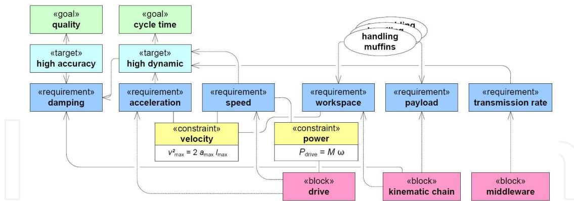
Fig. 4. Elements of an extended requirements diagram based on SysML.
