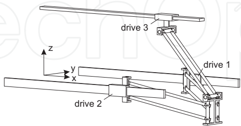
Fig. 9. Kinematic structure of the TRIGLIDE robot.
