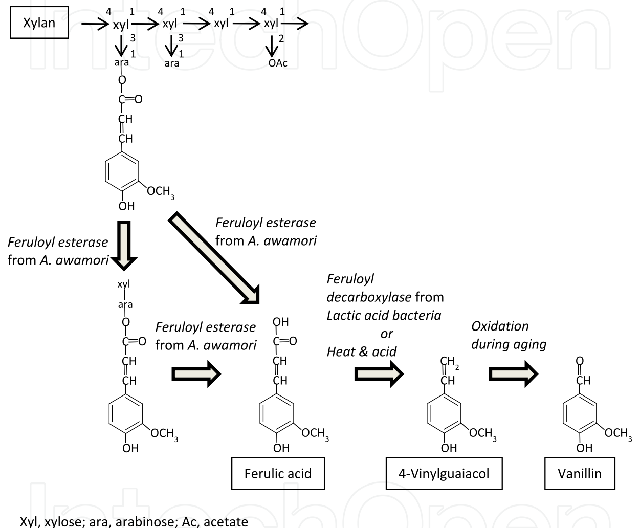
Fig. 5. Mechanisms of production of vanillin from ferulic acid during Awamori spirit
