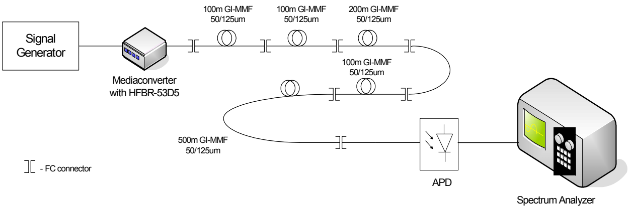
Fig. 19. Bandwidth measurement setup – a patchcord cascade.
