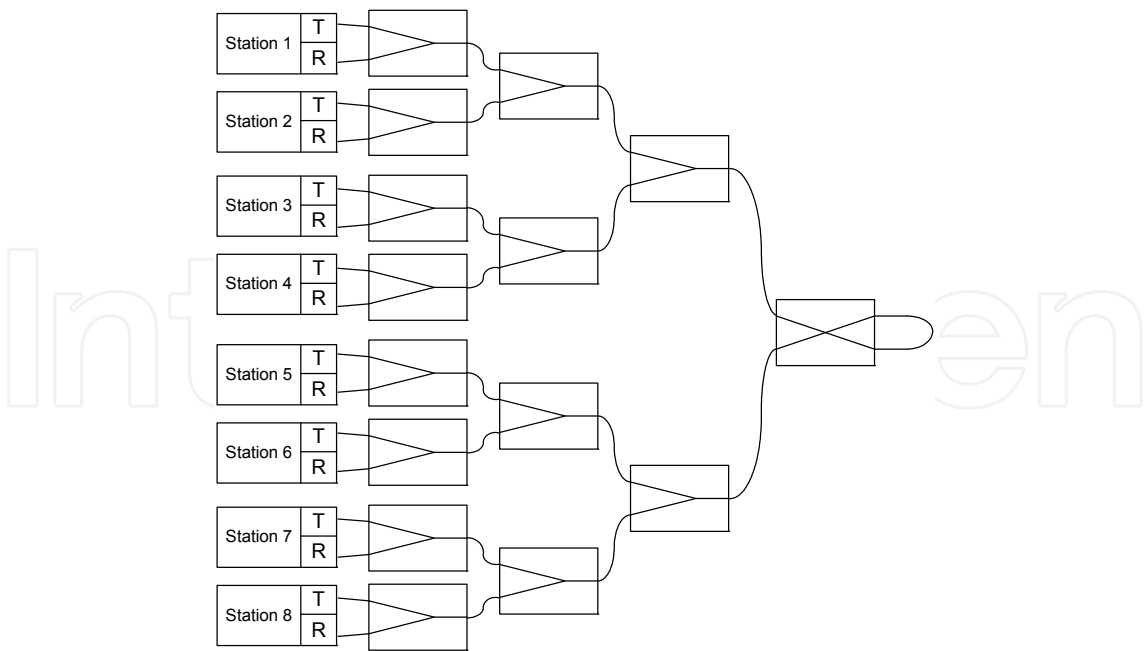
Fig. 3. Reflective star with 8 nodes.
