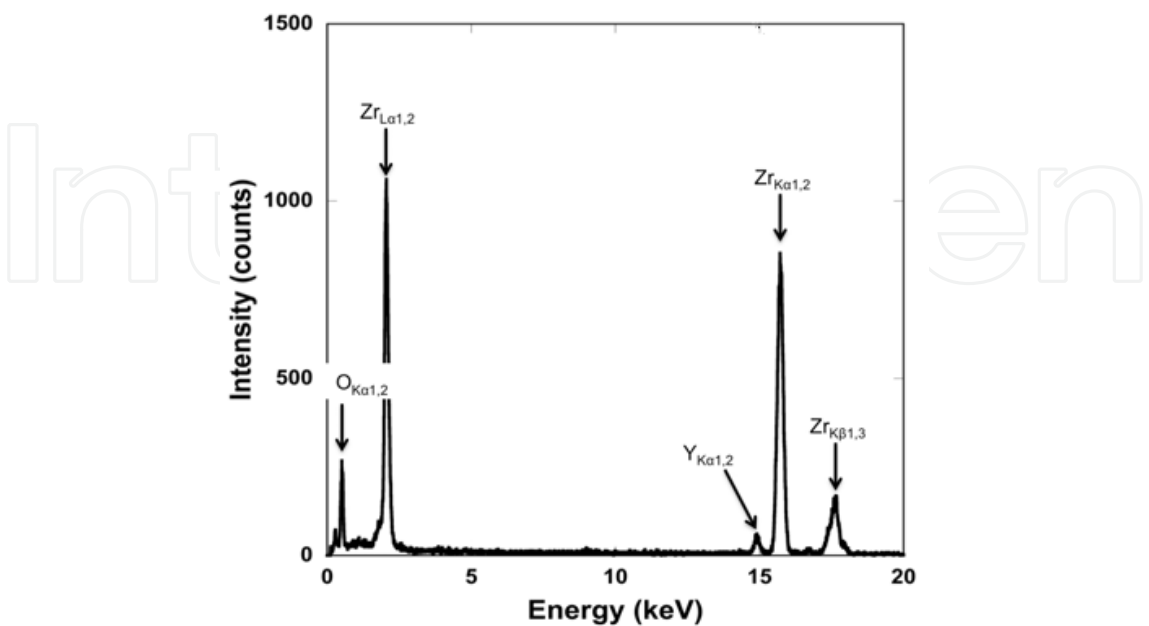
Fig. 3. Typical EDS profile obtained from Y_2O_3 doped ZrO_2 .
