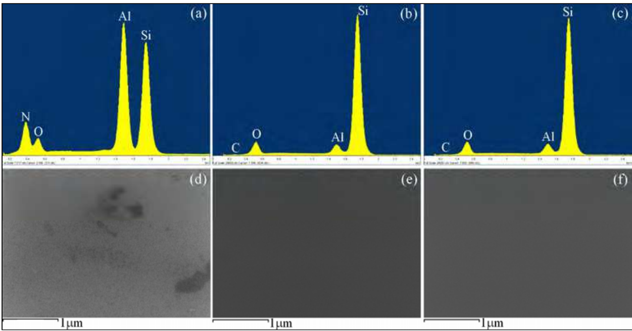
Fig. 6. EDS spectra and FESEM images of AlN thin films grown from metal target (a, d), ceramic target in Ar atmosphere (b, e) and ceramic target in a mixture of Ar and N 2 (c, f).
