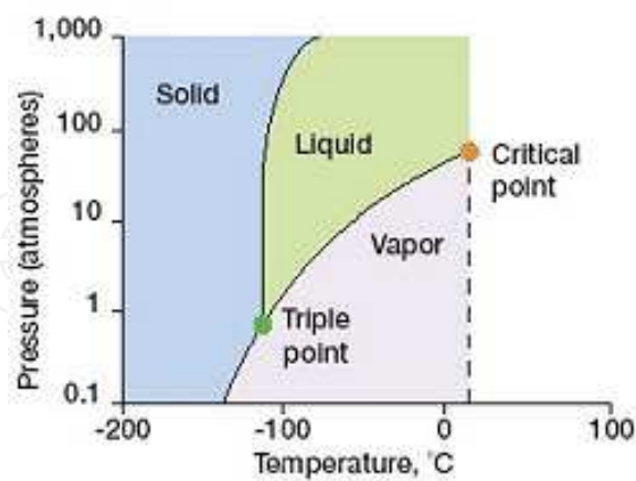
Fig. 1. Phase diagram of xenon. (Figure from: http://science.nasa.gov/science-news/science-at-nasa/2008/25apr_cvx2/ )
