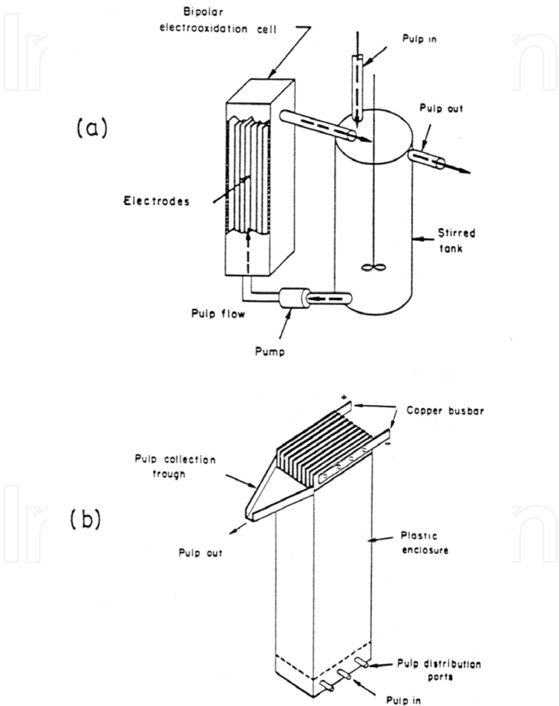
Fig. 8. Pulp flow sequence through agitator and bipolar cell (a), and electrooxidation electrode design (b) (from ref. 26)
