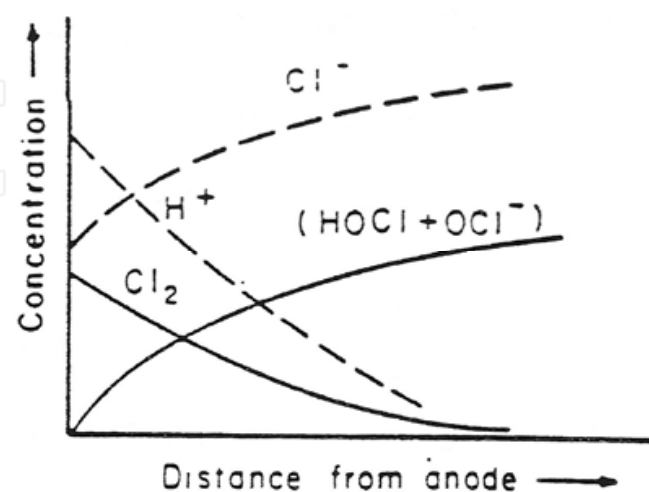
Fig. 4. Schematic representation of concentration profile near anode during the electrolysis of NaCl solution (10).
