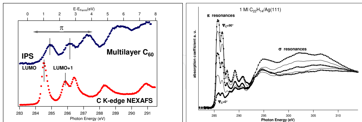
Fig. 4. Left: C Kedge NEXAFS of C 60 multilayer compared with Inverse Photoemission (Felici 2009). Right: Example of C Kedge NEXAFS of the linear molecule Pentacene (C 22 H 14 ) deposited (1ML) onto Ag(111) measured varying Electric field vector of the incident synchrotron light (Pedio 2007).
