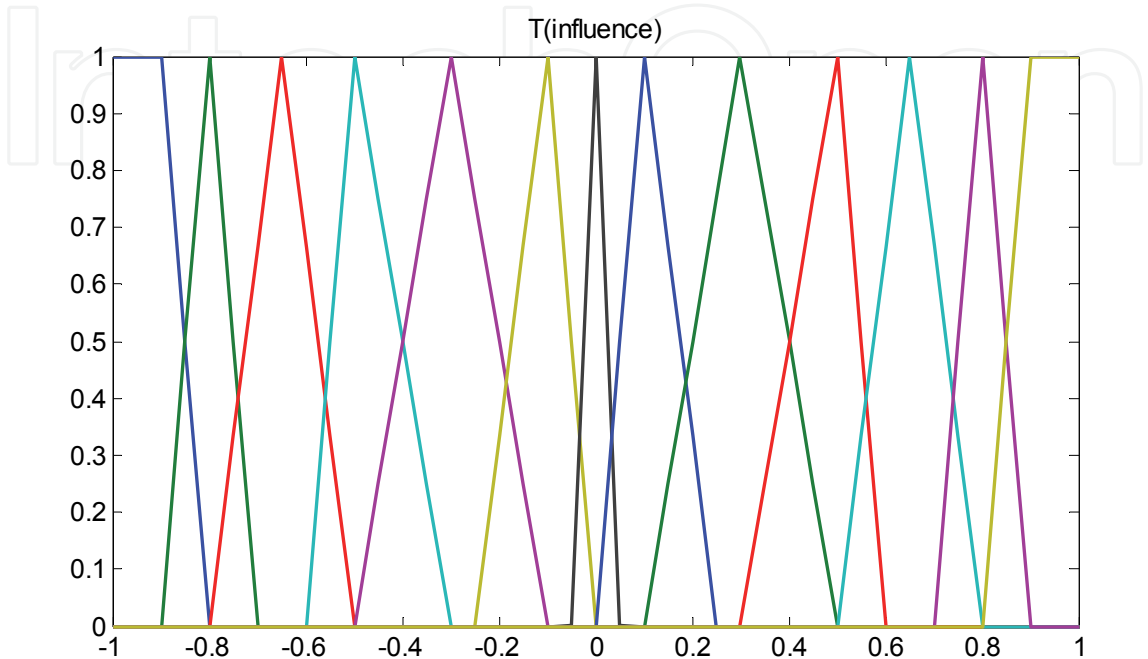
Fig. 2. The thirteen membership functions describing T(influence)
