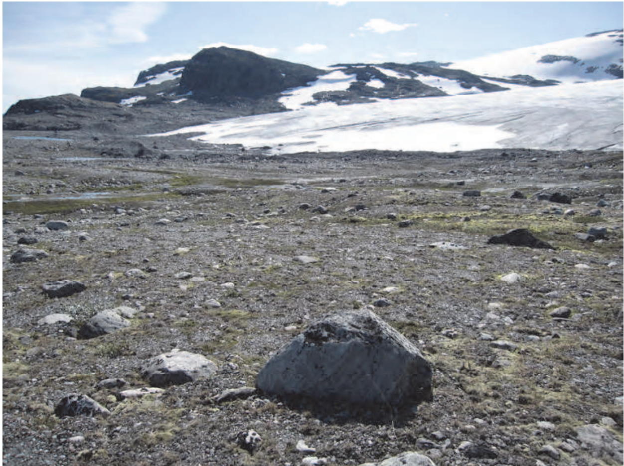
Fig. 1. Foreland at the Midtdalsbreen glacier snout, a part of the Hardangerjøkulen glacier in central south Norway. Photo: Sigmund Hågvar.
