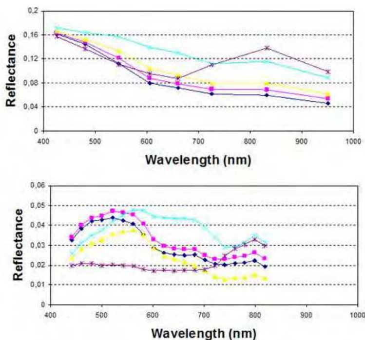
Fig. 5. Worldview-2 (top) and MIVIS (bottom) spectral profiles of water classes.
