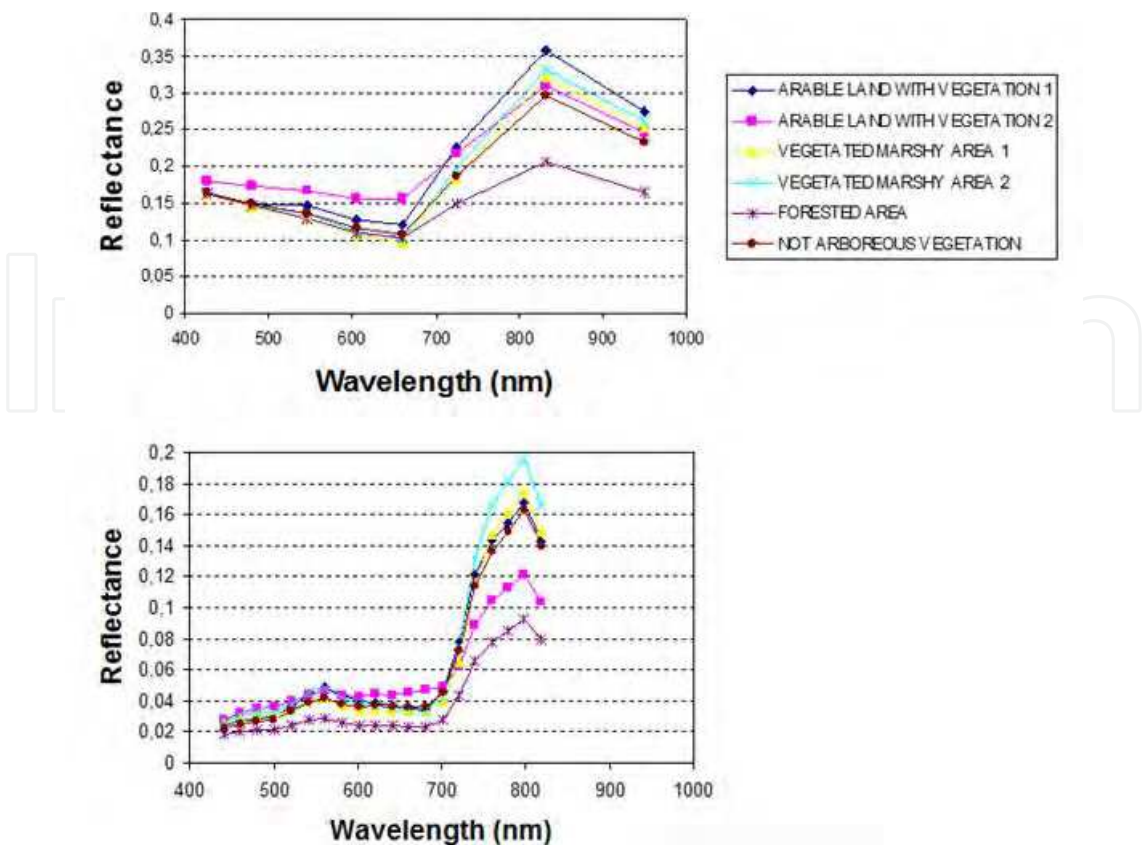
Fig. 7. Worldview-2 (top) and MIVIS (bottom) spectral profiles of vegetated land classes.
