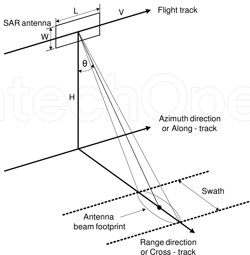
Fig. 2. Basic geometry of imaging SAR.
