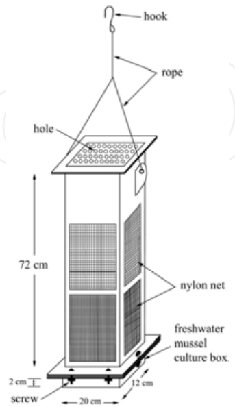
Fig. 3. Rearing container of juveniles (Kovitvadhi et al., 2006).
