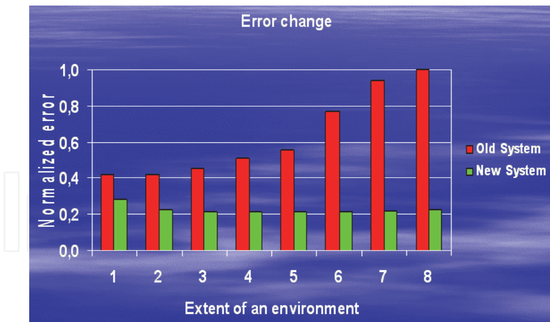
Fig. 5. Normalised error of measurement, depending upon the length of the path sounding.
