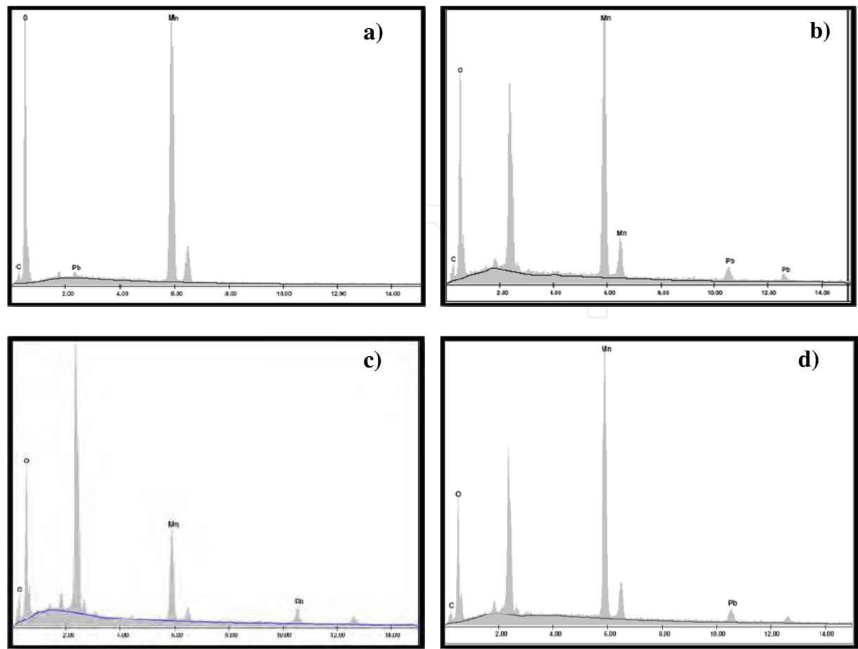
Fig. 6. EDX analysis conducted on surface: a) initially covered by manganese oxide and b) polished Mn; both during 24 h. c) Initially covered by manganese oxide and d) polished Mn; both during one week.
