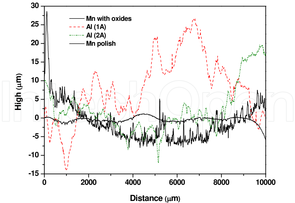
Fig. 22. Aluminum deposits profilometry from samples starting with polished and oxide surfaces.
