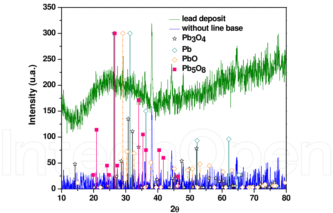
Fig. 7. X-ray diffraction of a lead deposit.
