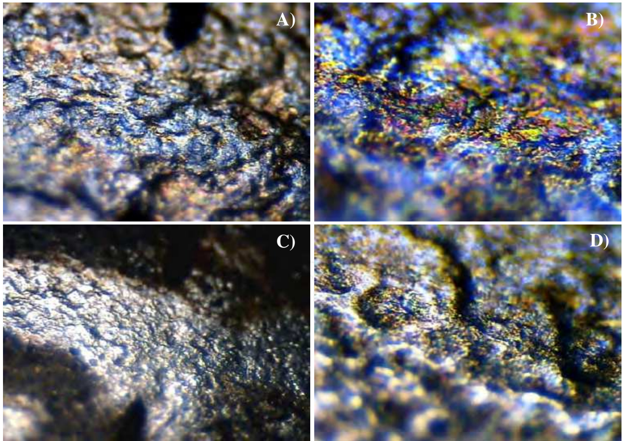
Fig. 21. Images of aluminum deposit on manganese-manganese oxide. A) and B) corresponds to a deposit on mangense-manganese oxide as susbtrate at 70 and 700x, respectively; C) and D) corresponds to a deposit on manganese with an ititially polished surface at 70 and 700x, respectively.
