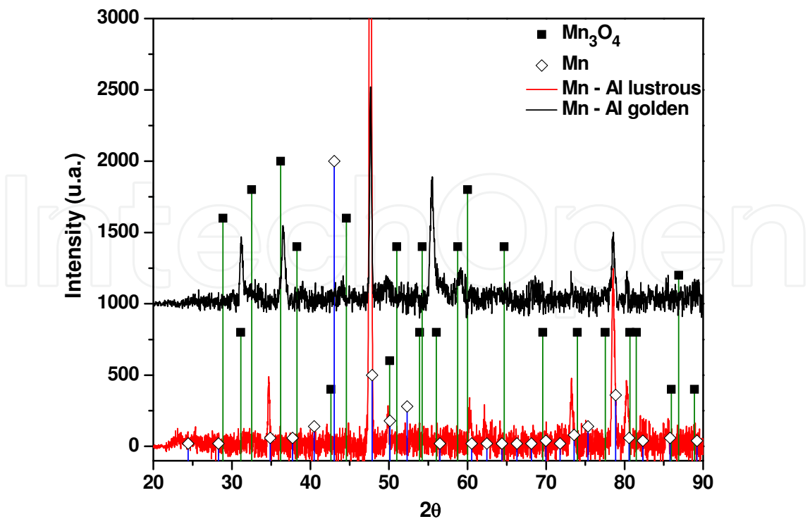
Fig. 17. Diffractogram of aluminum deposit on manganese substrate.
