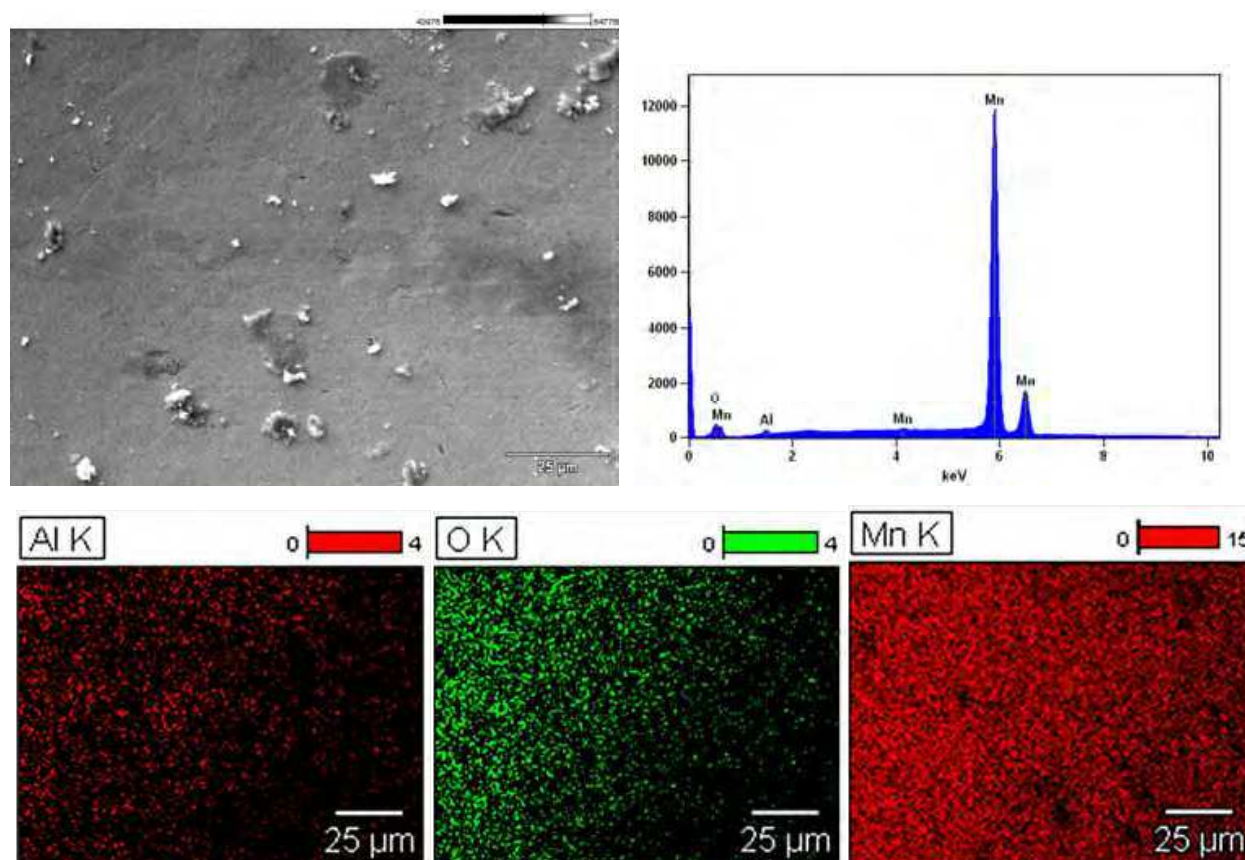
Fig. 19. SEM micrograph of the Aluminum deposit using 1000X (the scale bar indicate 25µm). Also, EDS microanalysis shows Mn, O and Al on surface. In the second line, the composition distribution maps on surface corresponding to Al, O, and Mn, respectively.
