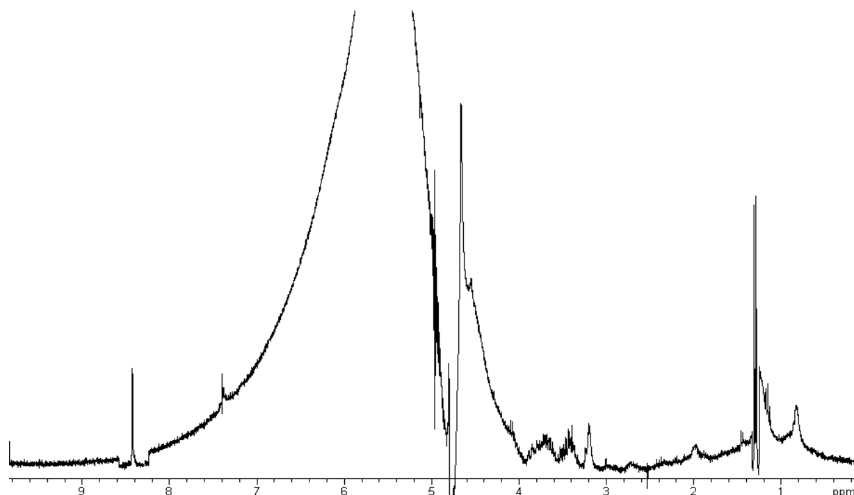
Fig. 9. 1 H-NMR spectrum of blood plasma of mouse after acute hypoxia at 4.2% pO 2 during 10 min.
