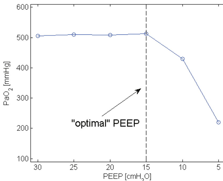
Fig. 5. Change of \text{PaO}_2 during a decremental PEEP trial in a porcine model of acute lung injury. Vertical dashed line indicates the optimal PEEP level with respect to \text{PaO}_2 .
