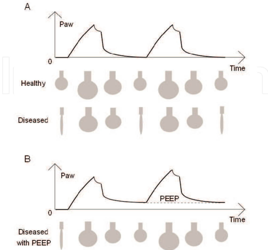
Fig. 4. The effect of positive end-expiratory pressure (PEEP) on keeping the alveoli open. A: Under controlled mechanical ventilation without PEEP, alveoli of a healthy subject stay open throughout the whole breathing cycle, while the alveoli of a patient with lung disease collapse at the end of expiration. B: When PEEP is applied, the recruited alveoli will no longer collapse at the end of expiration in a patient with lung disease.
