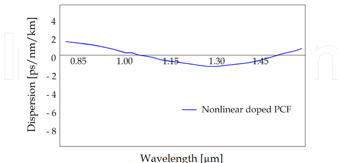
Fig. 3. Chromatic dispersion in regular solid-core PCF and modeled doped PCF.
