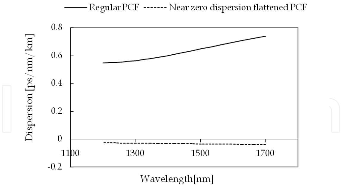
Fig. 8. Chromatic dispersion of the designed PCF compared to the regular IGPCF.
