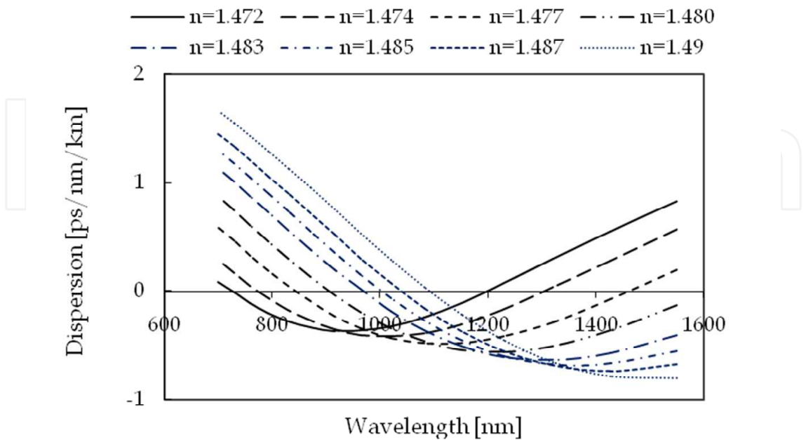
Fig. 6. Chromatic dispersion dependence on dopant material refractive index.
