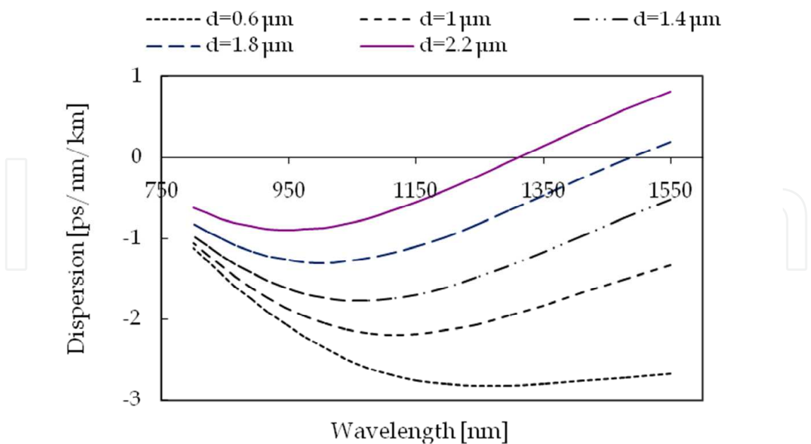
Fig. 4. Chromatic dispersion dependence on hole diameter.
