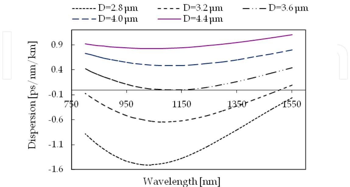
Fig. 5. Chromatic dispersion dependence on core diameter.
