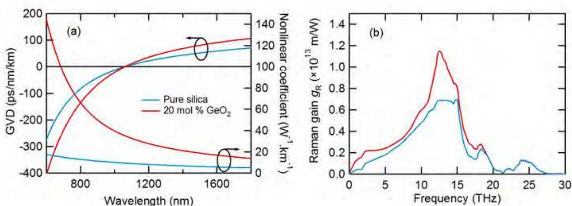
Fig. 11. (a) GVD curves (left axis) and nonlinear coefficient (right axis) calculated for a pure silica PCF (blue) and a PCF doped with a \text{GeO}_2 content of 20 mol.%. (b) Raman gain spectra g_R for pure silica (blue) and 20 mol.% \text{GeO}_2 -doped silica (for a 164 nm pump).
