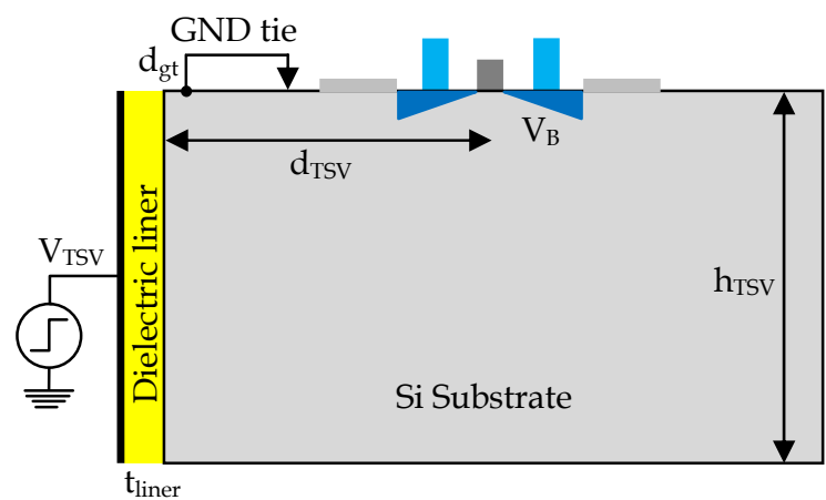
Fig. 5. Cross-section view of TSV-to-device coupling (Khan, 2009, 2011).
