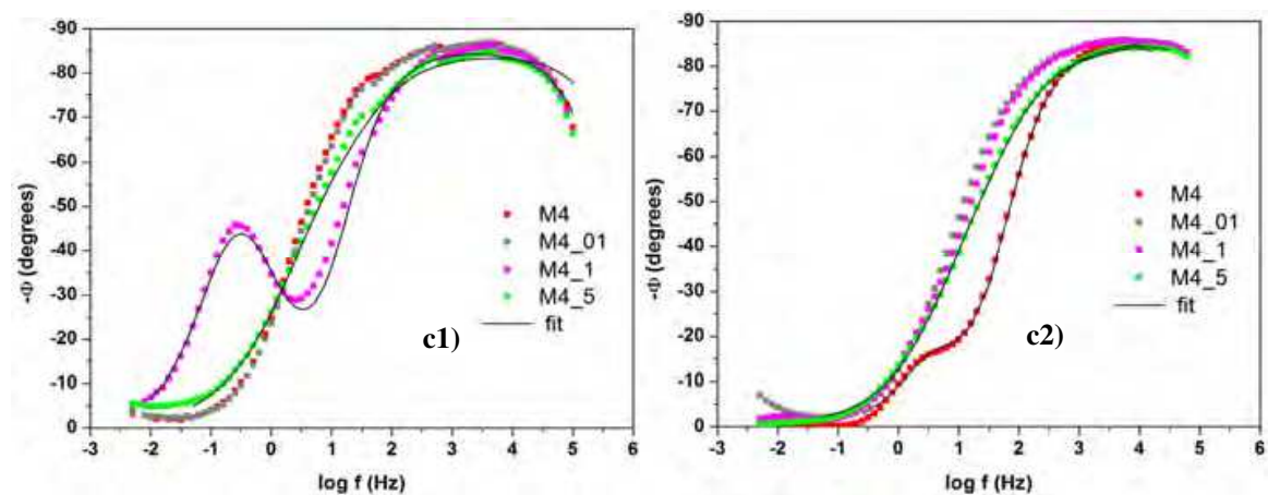
Fig. 15. Complex plane impedance (a), modulus impedance (b) and phase (c) plots of bare carbon steel and hybrids prepared with a MMA/MPTS a ratio of 4 containing CNTs with [C CNT ]/[C CNT + Si] molar concentrations of 0% (M4), 0.1% (M4_01), 1.0% (M4_1) and 5% (M4_5) after exposure of 1 day in (1) unstirred and naturally aerated 3.5 % NaCl and (2) 0.05 mol L -1 NaCl + 0.05 mol L -1 H 2 SO 4 solutions. (The small discontinuities of \theta vs. log f mark the change of the measurement range of the instrument.)
