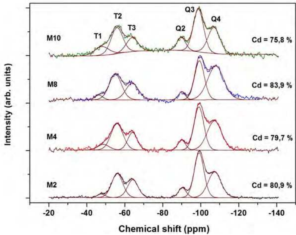
Fig. 3. 29 Si NMR spectra of hybrids prepared with MMA/MPTS ratios of 2 (M2), 4 (M4), 8 (M8) and 10 (M10).
