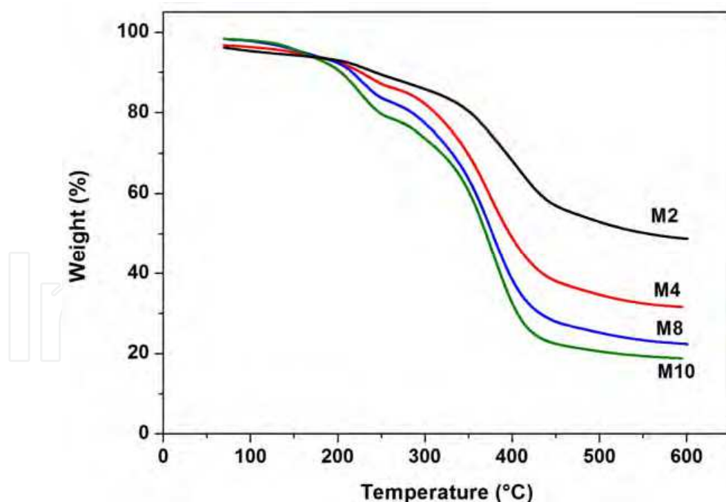
Fig. 4. TGA and DTG (insert) curves of hybrids prepared with MMA/MPTS ratios of 2 (M2), 4 (M4), 8 (M8) and 10 (M10).
