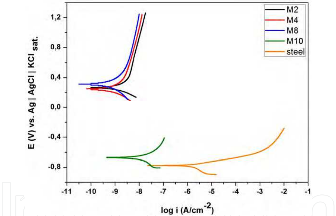
Fig. 9. Potentiodynamic polarization curves of bare carbon steel and hybrids prepared with MMA/MPTS ratios of 2 (M2), 4 (M4), 8 (M8) and 10 (M10) recorded after 2 h immersion in unstirred and naturally aerated 3.5 % NaCl solution.
