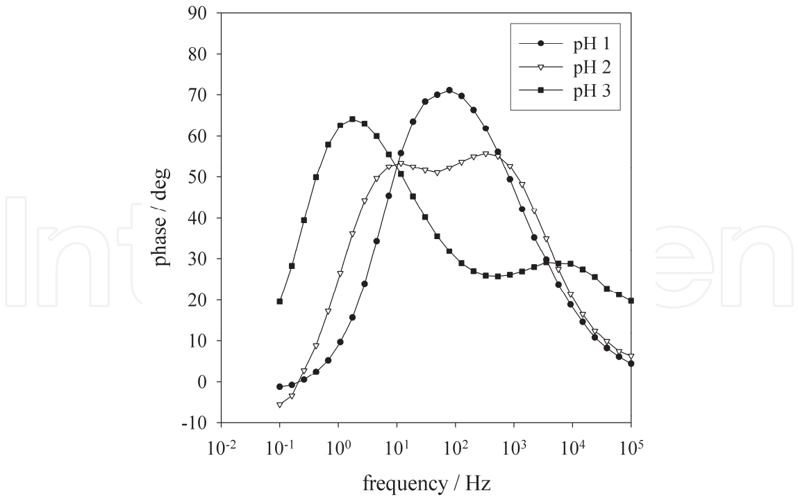
Fig. 14. Bode-phase diagrams at different pH of the sulphate electrolyte solution. Aluminium samples coated without pre-treatment; data obtained after 48 h of exposure to humidity chamber and 4 h of immersion in the electrolyte solution [48].
