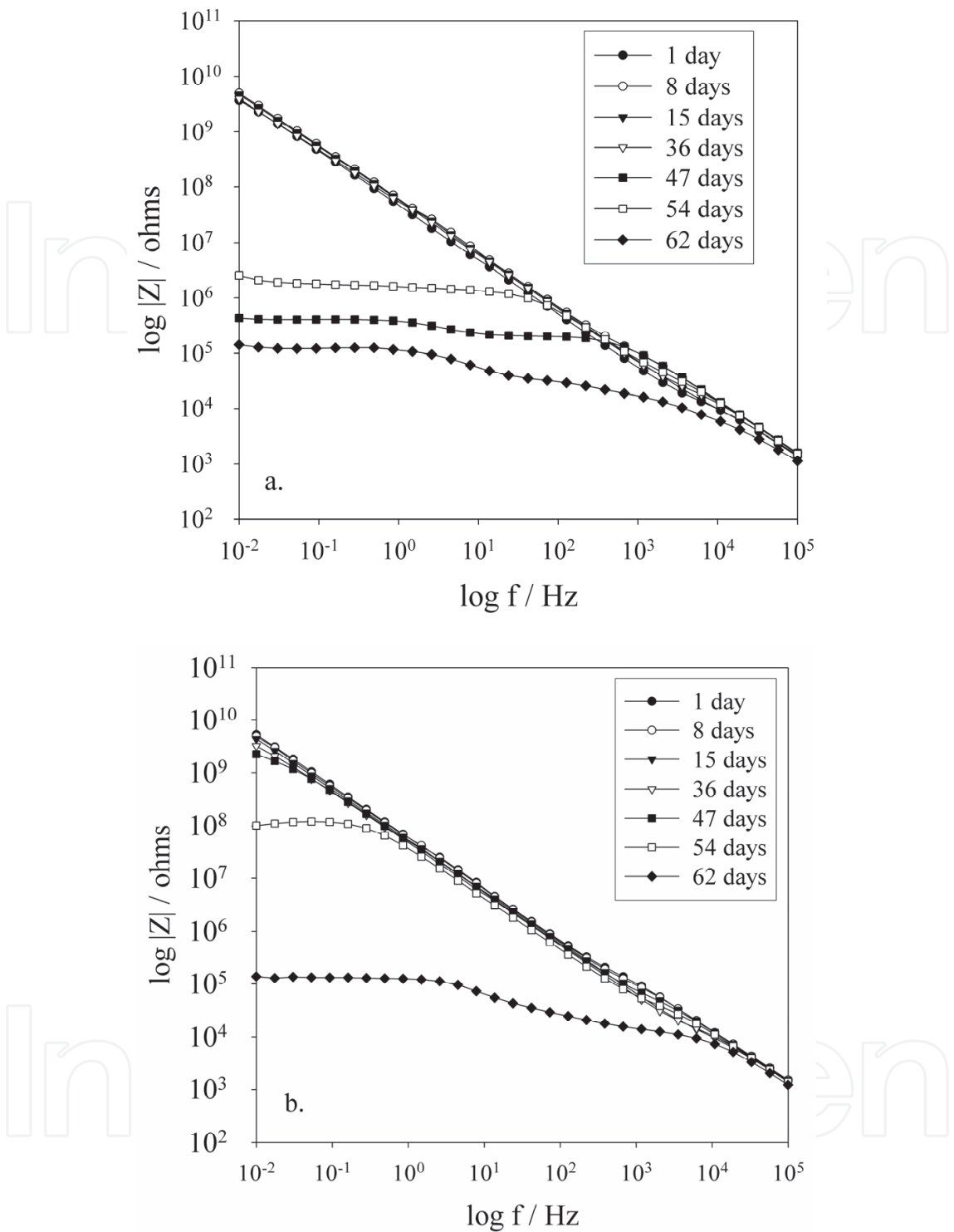
Fig. 6. Bode-modulus plots for different immersion times in NaCl 0.5 M of electrocoated aluminium samples without pre-treatment (a) and with a Zr/Ti pre-treatment (b) [36].
