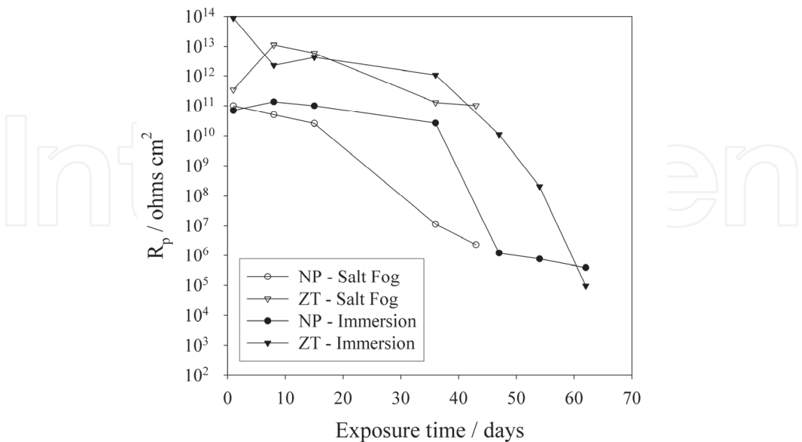
Fig. 7. Pore resistance as a function of exposure time to salt fog or to an immersion test for NP and ZT samples [36].
