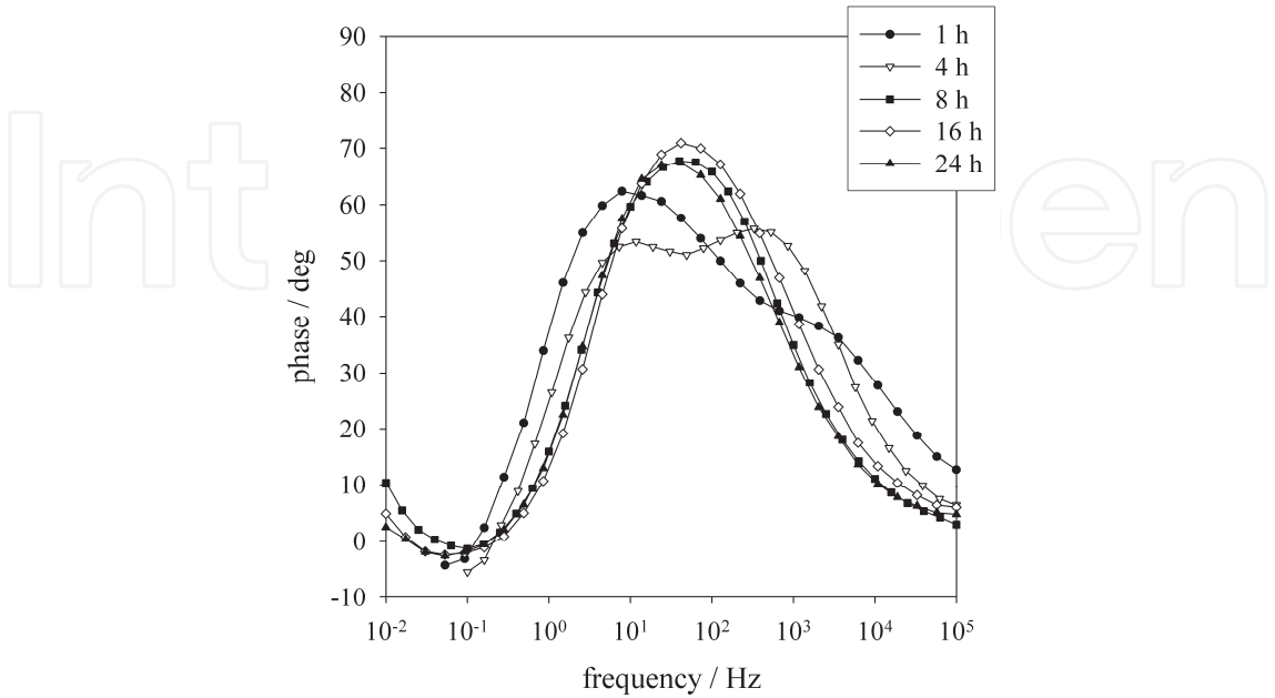
Fig. 13. Bode-phase diagrams for different immersion times in the sulphate electrolyte solution at pH 2. Data obtained with aluminium samples etched and electrocoated without any pre-treatment; exposure time in the humidity chamber: 48 h [48].
