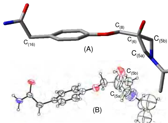
Fig. 15. (A) Geometry of (R,S)-atenolol in the crystalline structure showing the two alternative positions for the C 5 carbon atom; (B) ORTEP drawing (30% displacement ellipsoids) showing the thermal motion disorder exhibited by the tail fragment.
