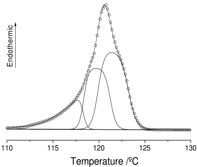
Fig. 5. Peak-fitting analysis of the fusion curve of the most stable form of erythritol. Values of T_{max} for the decomposed peaks are given in Table 2. Reprinted from International Journal of Pharmaceutics, Vol 388, A.J. Lopes Jesus et. al. / Erythritol: Crystal growth from the melt, Page 131, Copyright (2010), with permission from Elsevier.
