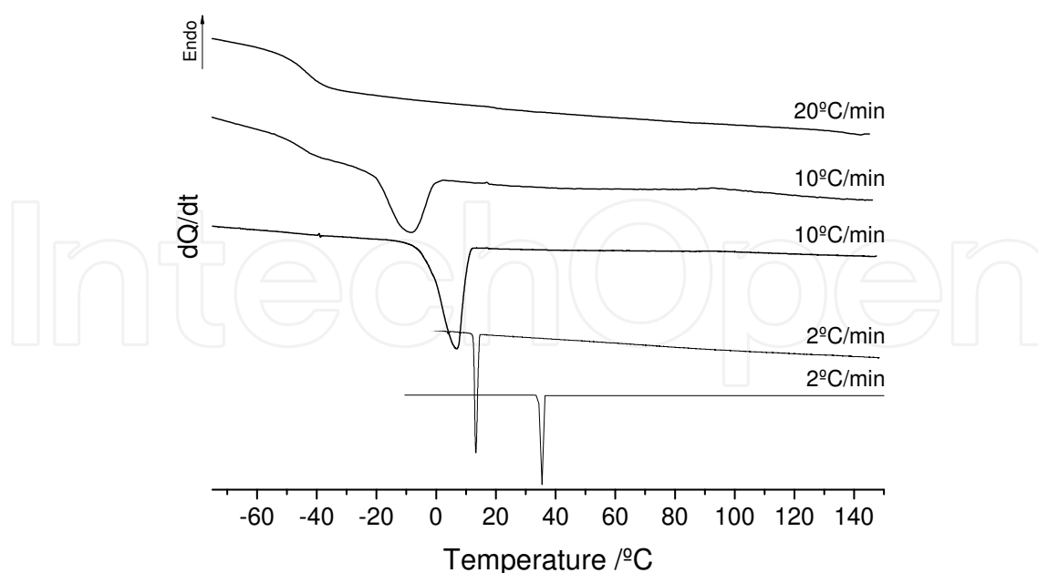
Fig. 3. DSC cooling curves of molten erythritol at different scanning rates. Reprinted from International Journal of Pharmaceutics, Vol 388, A.J. Lopes Jesus et. al. / Erythritol: Crystal growth from the melt, Page 130, Copyright (2010), with permission from Elsevier.
