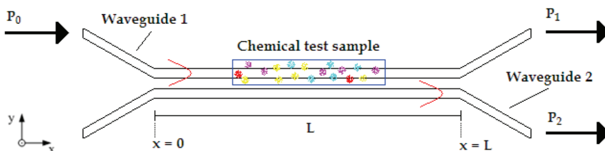
Fig. 18. Schematic representation of an integrated direction coupler.
