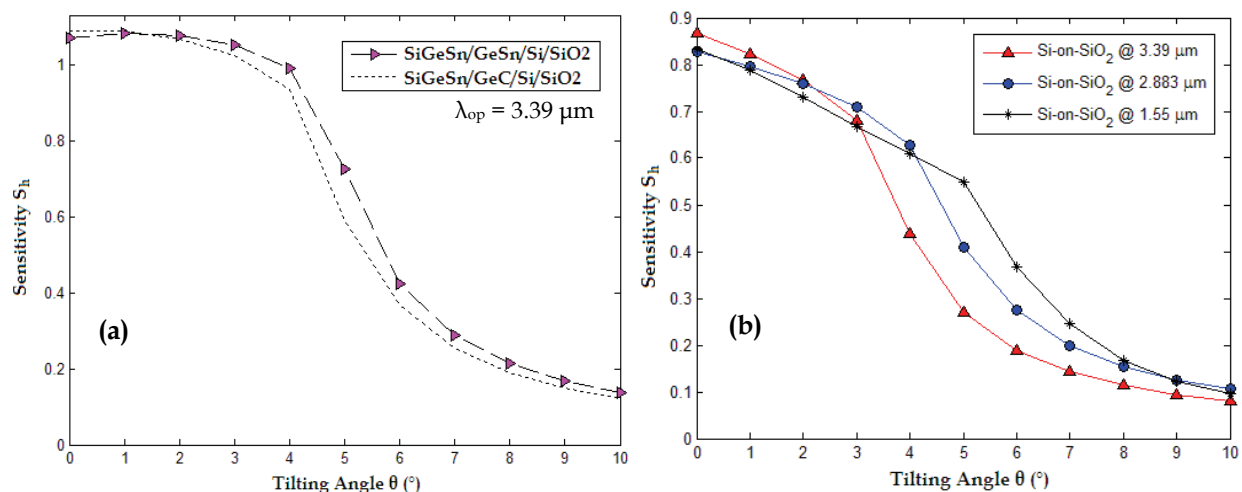
Fig. 10. Sensitivity of optimized slot waveguides as a function of the tilting angle \theta with slot region width g fixed at 100nm in all cases. (a) Tolerance analysis of group IV-based optimized slot waveguides presented in Fig. 8; (b) Tolerances analysis of conventional SOI slot waveguides (@ 1.55 \mu\text{m} , w = 230\text{nm} , h = 500\text{nm} , @ 3.39 & 2.883 \mu\text{m} , see also Fig. 7b).
