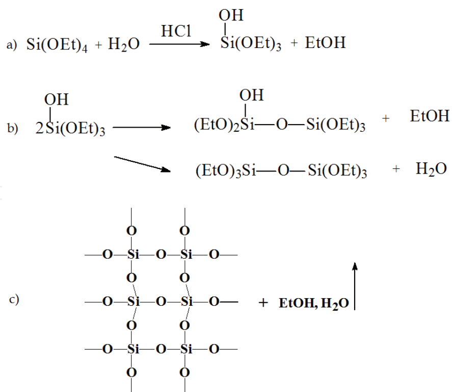
Fig. 6. The silica clusters preparation: (a) the hydrolysis catalyzed by the acid; (b) the condensation; (c) the alternating -Si-O-Si- containing clusters and further nanoparticles.
