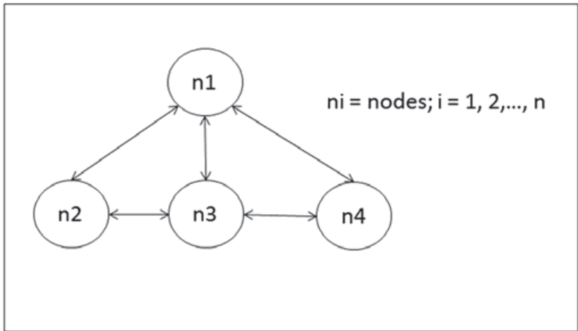
Fig. 11. Navigation tree.
